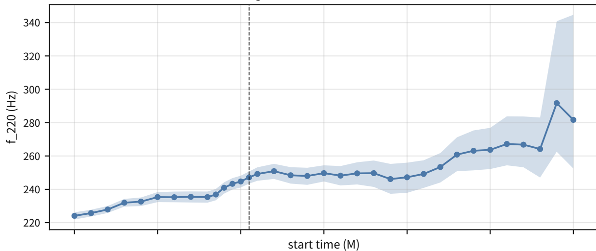
QNM f220 vs start time
