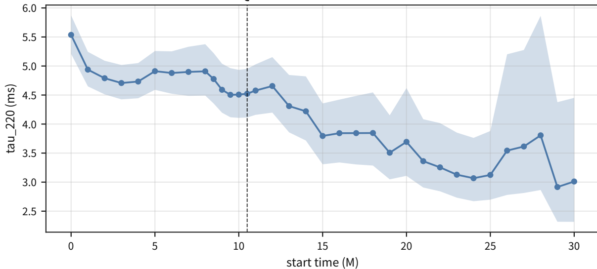
QNM tau220 vs start time
