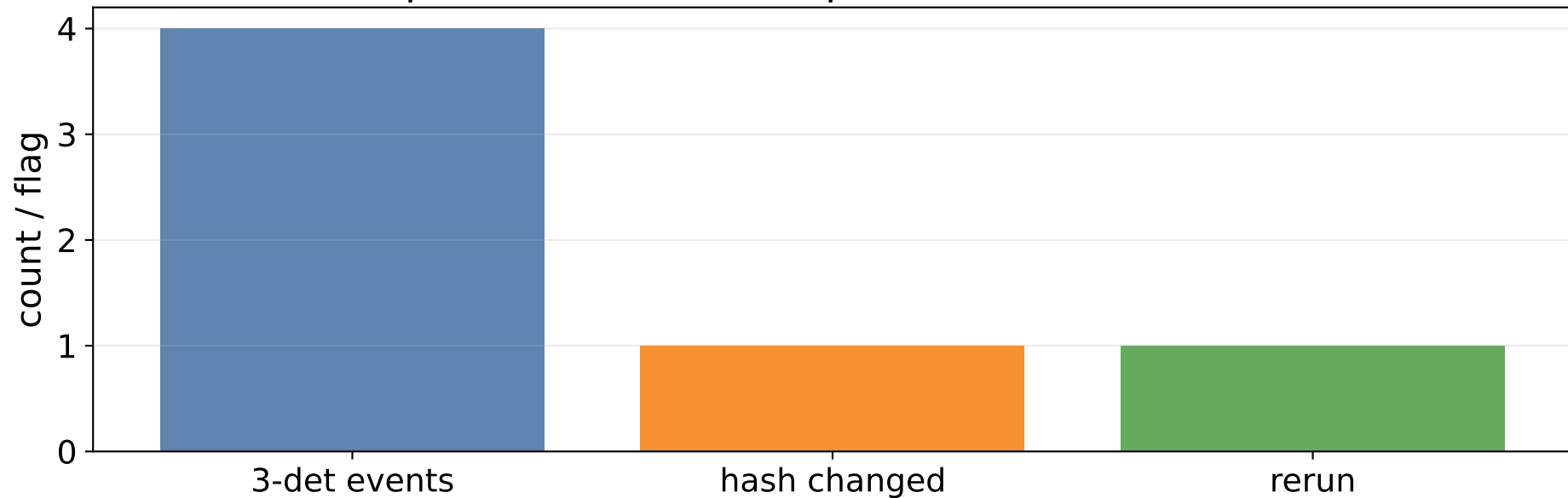
GW polarization event-update watch (3-detector)
