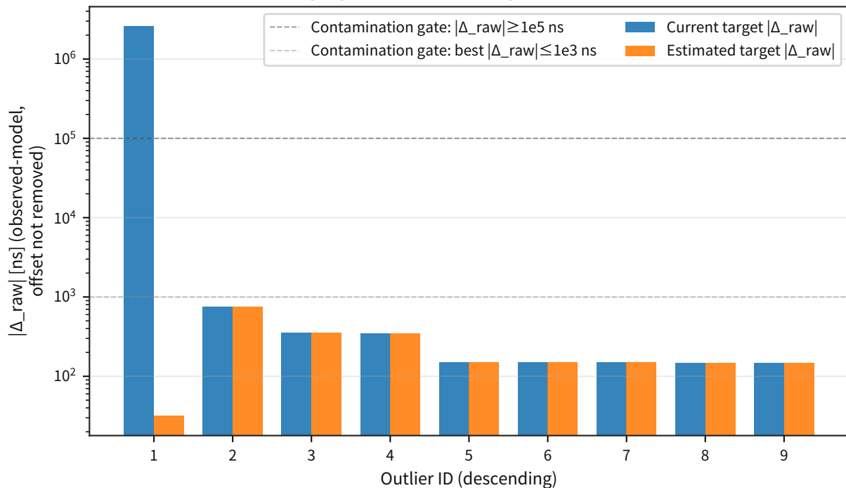
Lunar Laser Ranging (LLR): outlier target-contamination sensitivity
