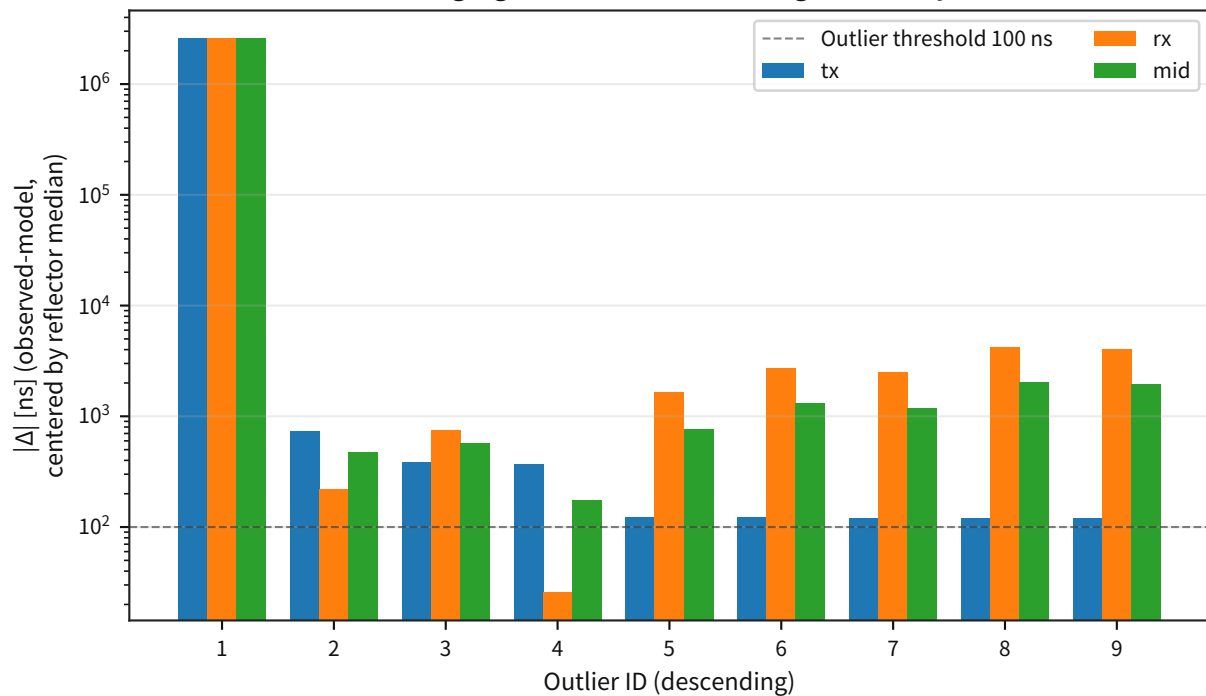
Lunar Laser Ranging (LLR): outlier time-tag sensitivity (tx/rx/mid)
