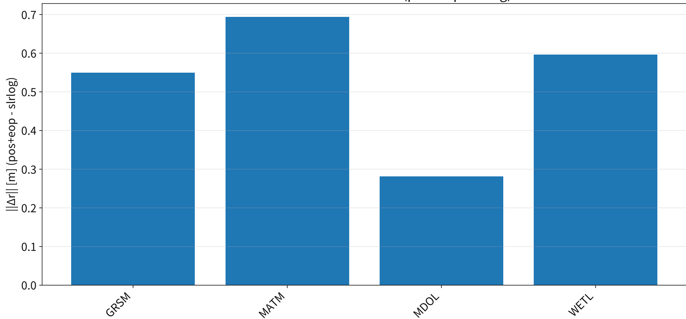
LLR: station-coordinate delta (pos+eop - slrlog)
