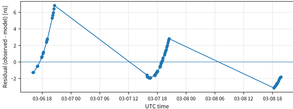
Residual after constant-offset alignment (reflector model, with solar Shapiro)
