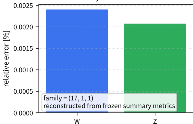
same-family mass-anchor errors
