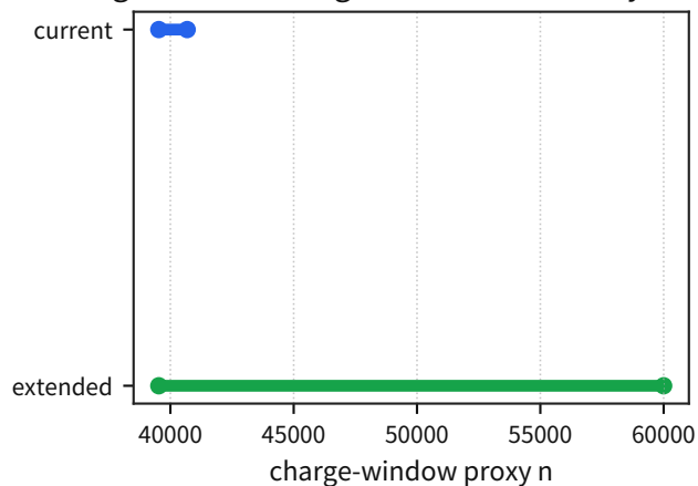
charge-window range used in the theory baseline
