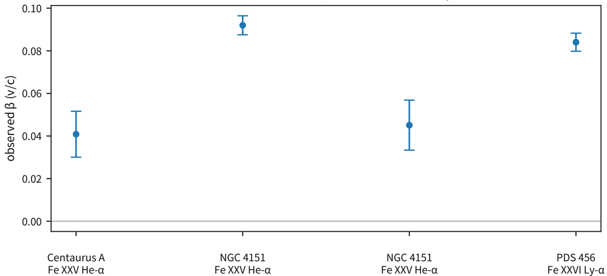
XRISM Resolve: BH/AGN line-centroid \beta
