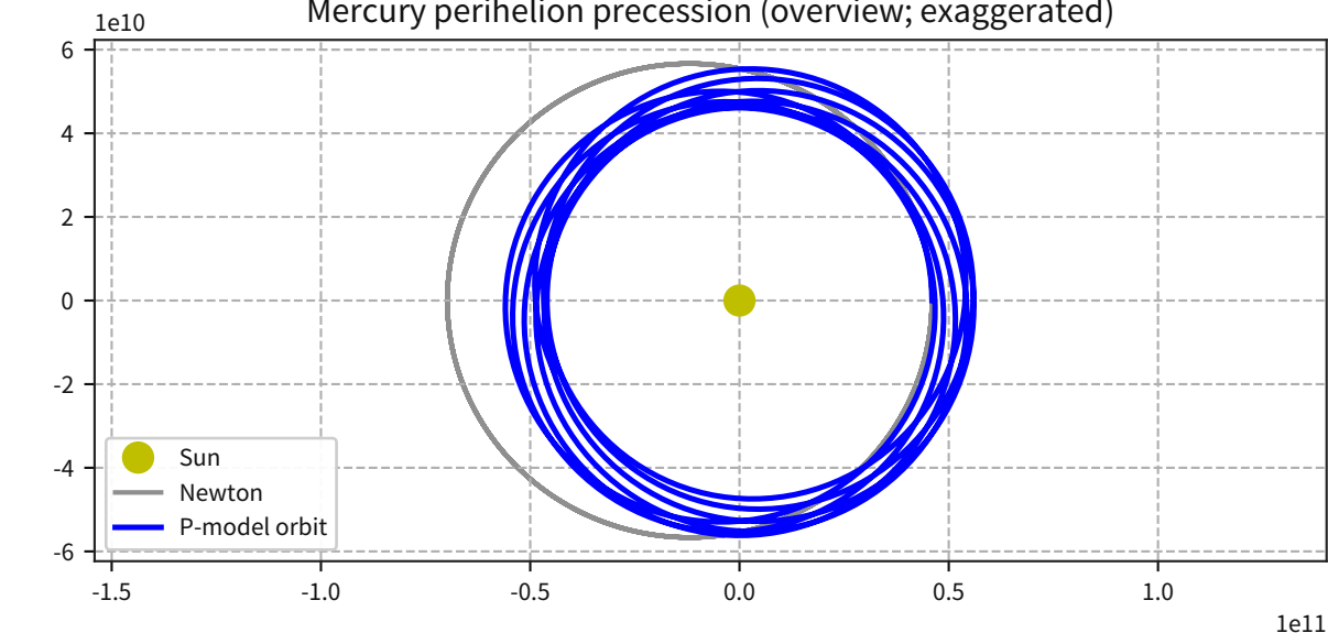
Mercury perihelion precession (overview; exaggerated)
