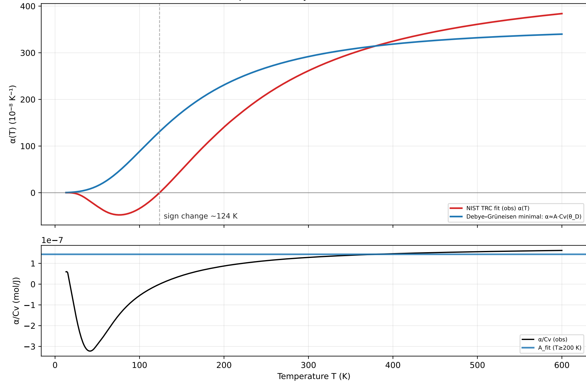
Silicon thermal expansion: Debye-Grüneisen minimal model check
