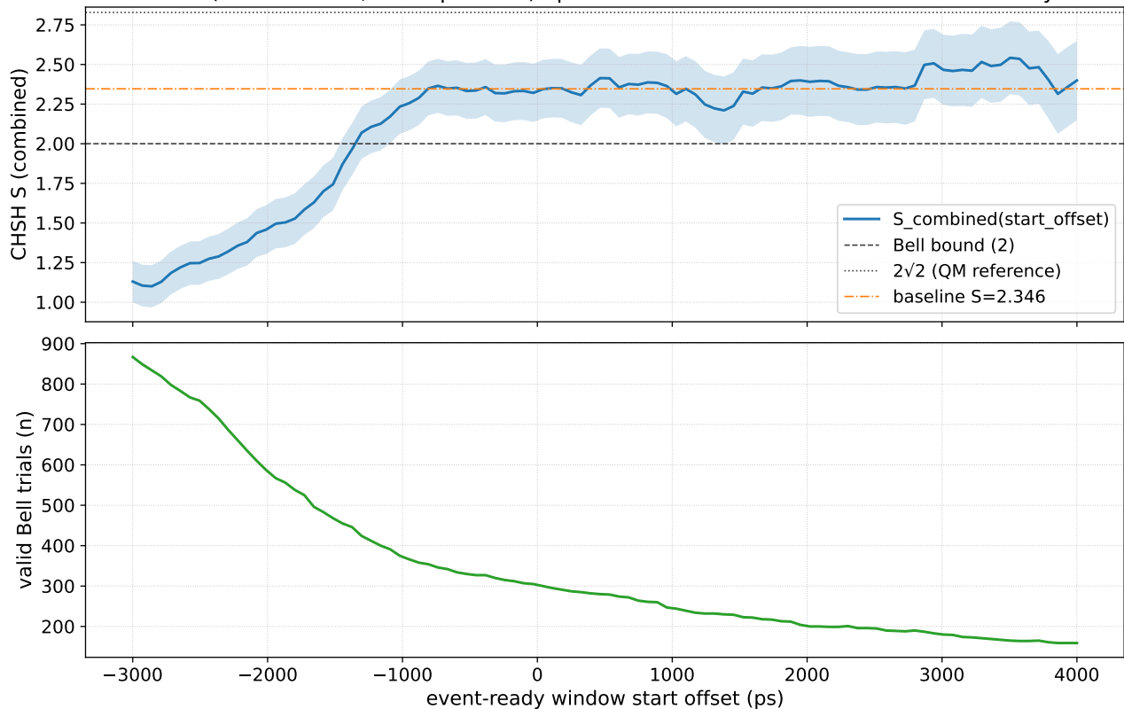
Delft (Hensen 2016; Sci Rep 30289) open data: CHSH S and window-start sensitivity
