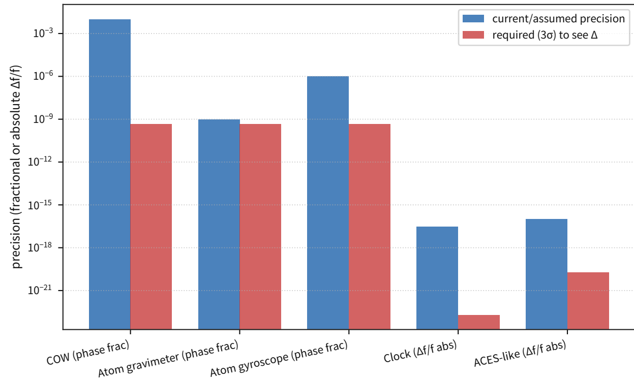
Atom-interferometer unified audit (P-model vs GR; Earth field)
