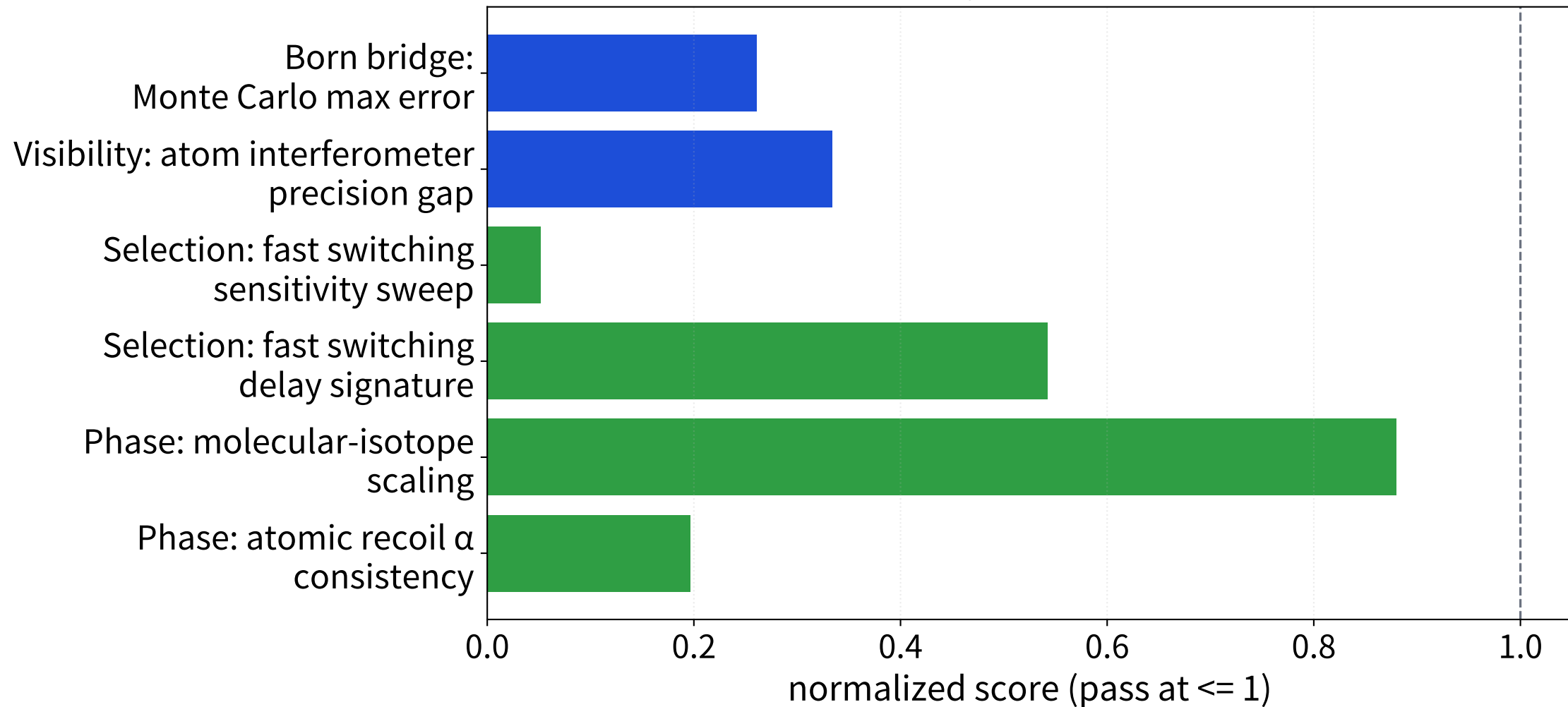
Born route-A proxy constraints (A continue)
