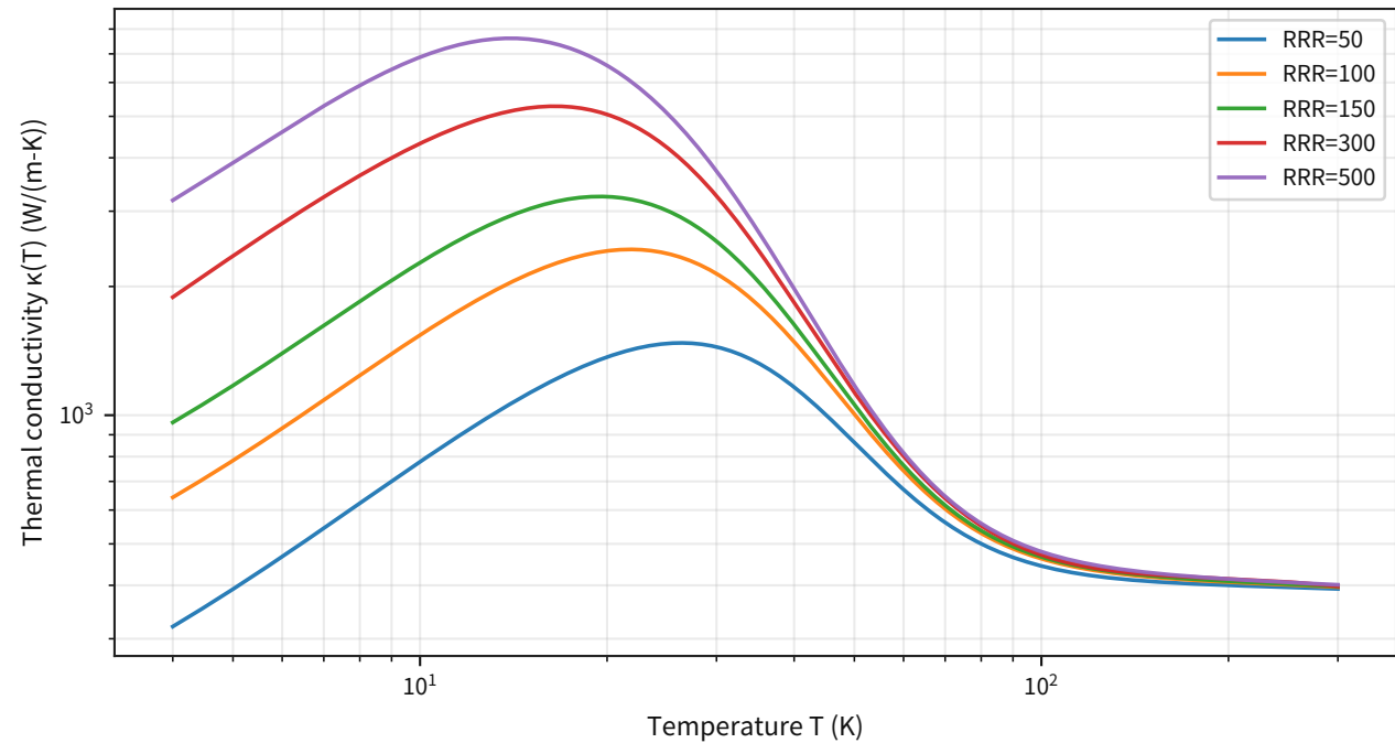
OFHC Copper thermal conductivity \kappa(T) (NIST TRC cryogenics fit)
