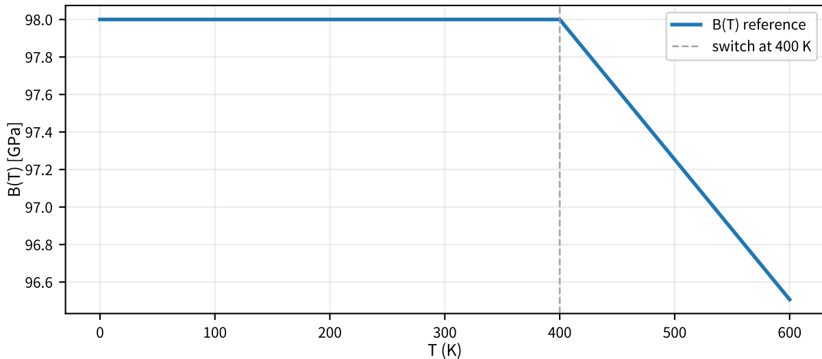
Silicon bulk modulus B(T) (Ioffe elastic constants reference)
