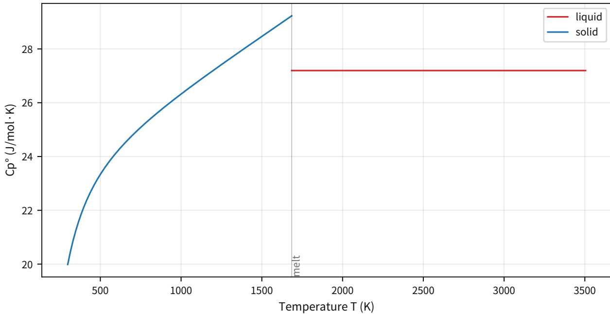
Silicon heat capacity (Shomate; NIST WebBook condensed phase)
