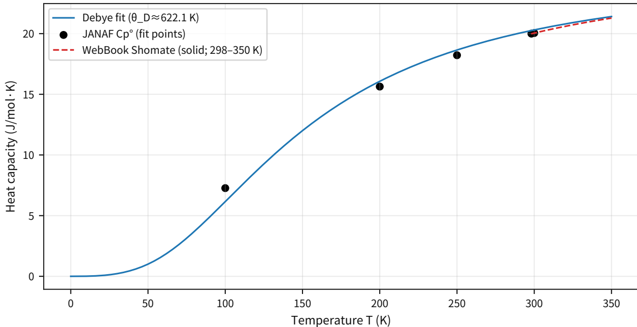
Silicon heat capacity: JANAF baseline + Debye-fit target (low T)
