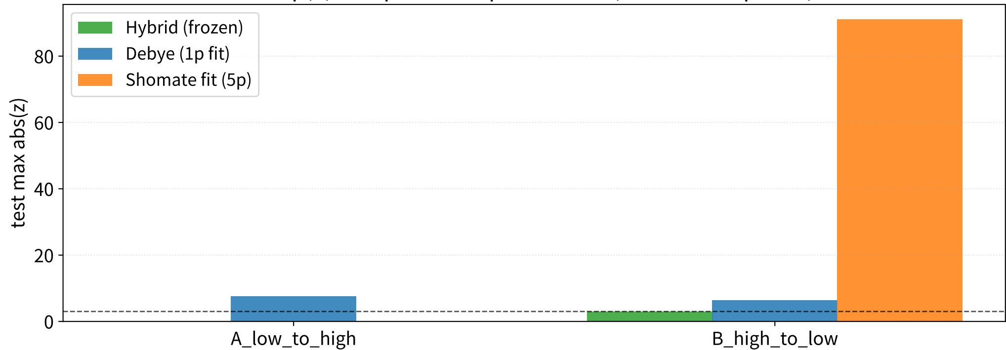
Si Cp(T): temperature-split holdout (JANAF solid points)
