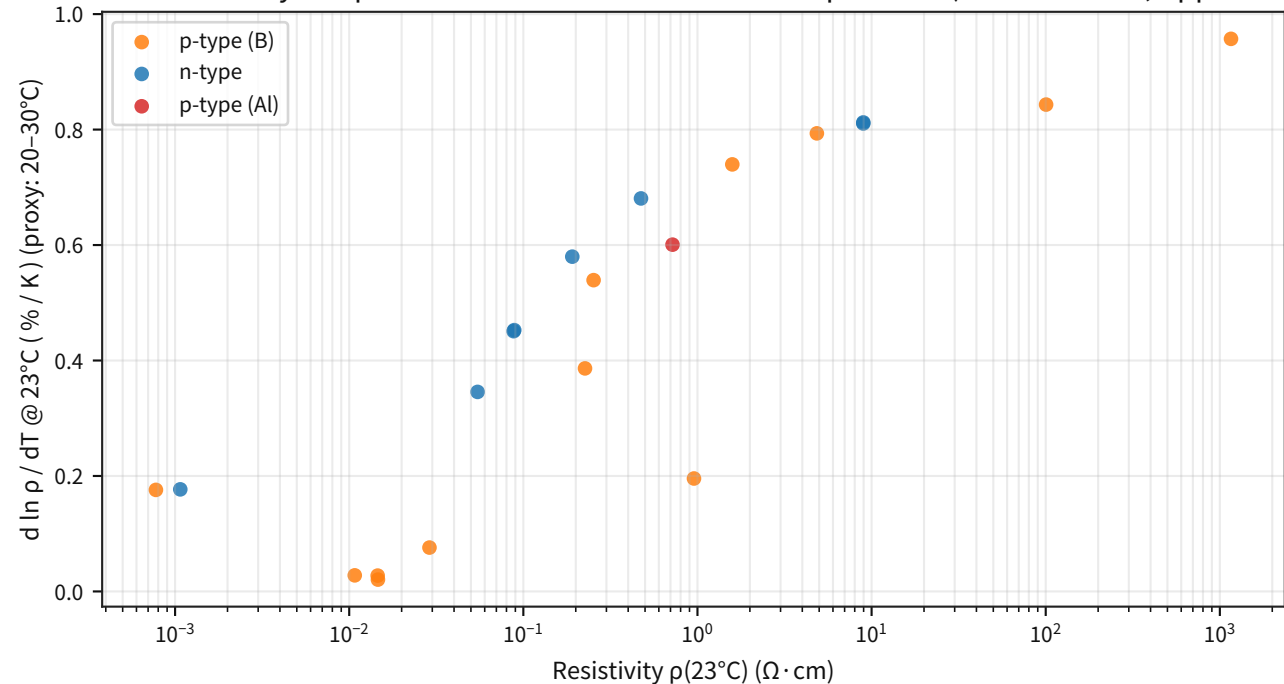
Silicon resistivity temperature coefficient near room temperature (NBS IR 74-496; Appendix E)
