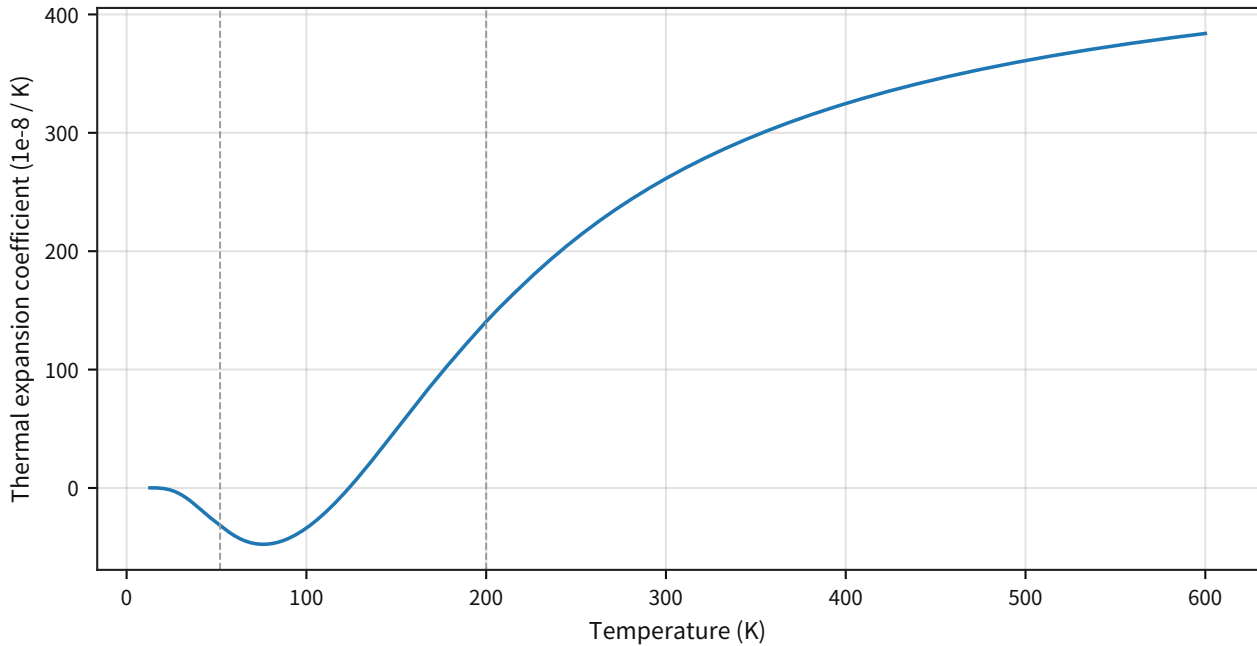
Si thermal expansion coefficient (NIST TRC fit)
