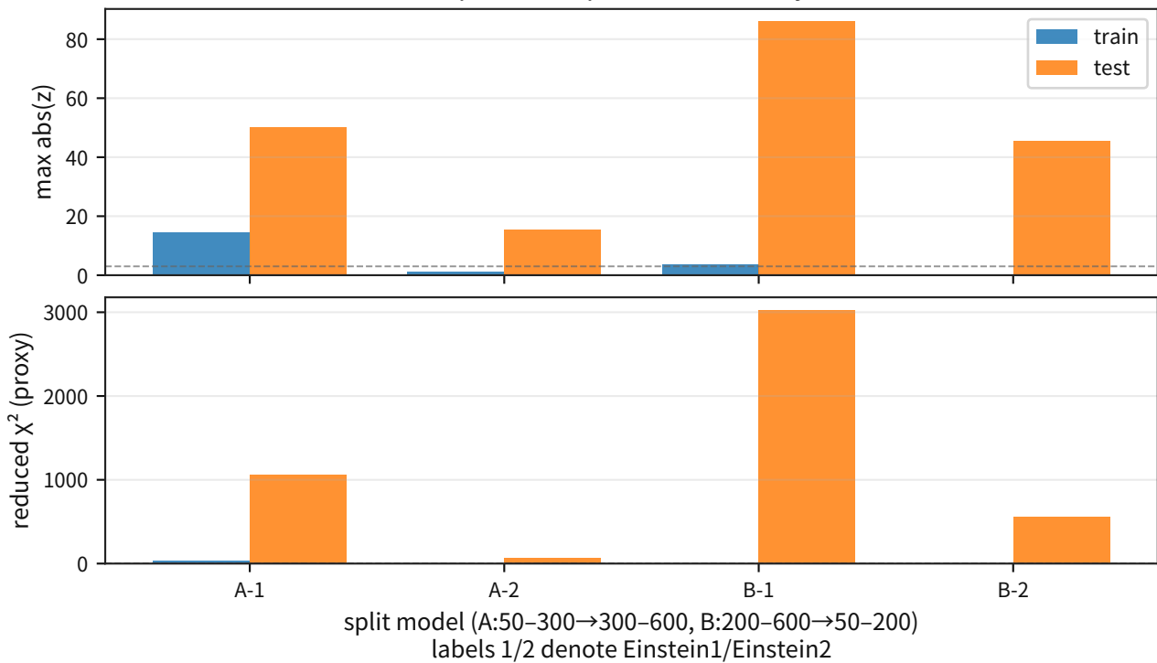
Si \alpha(T) : temperature-split holdout (Debye+Einstein)
