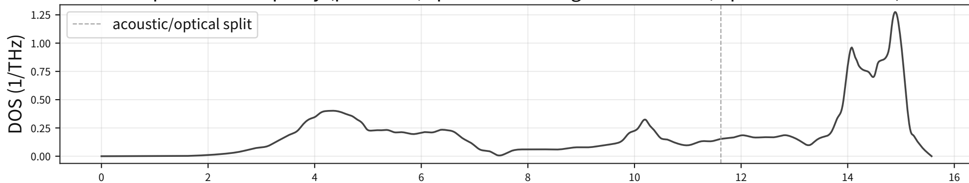
Si phonon DOS proxy (per atom; split at half-integral \approx acoustic/optical mode count)
