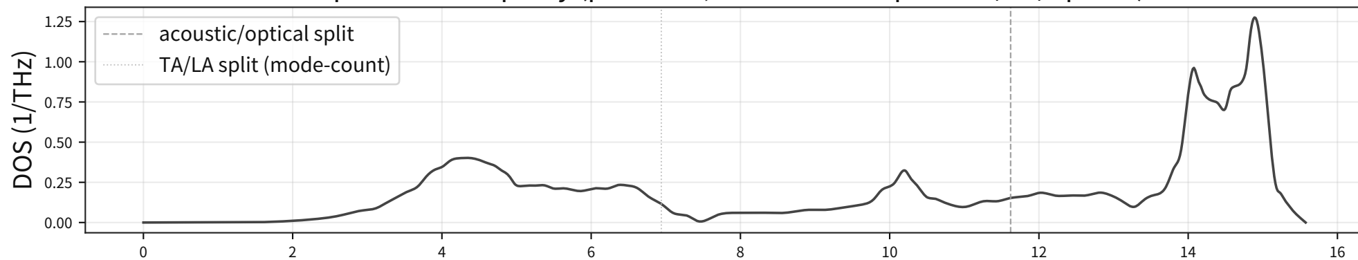
Si phonon DOS proxy (per atom; mode-count splits: TA/LA/optical)
