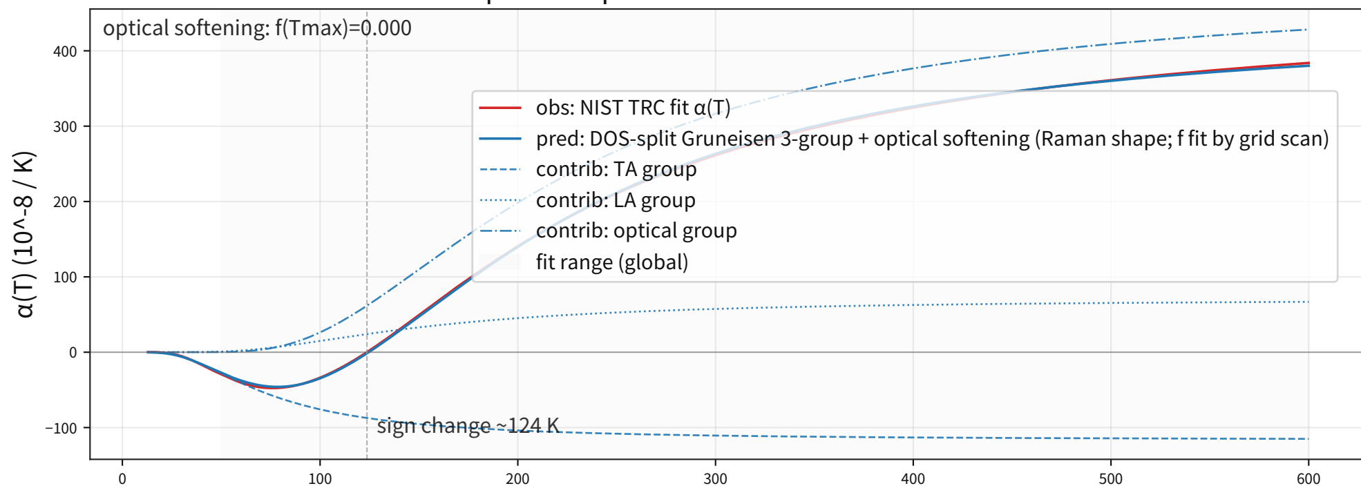
Si thermal expansion: phonon DOS constrained Gruneisen check
