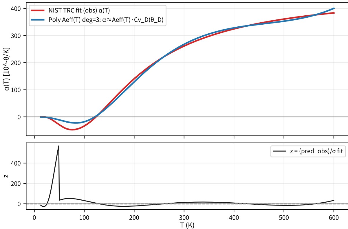
Silicon thermal expansion: polynomial Aeff(T) ansatz (diagnostic)
