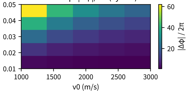
H-v sweep: |\Delta\phi|/2\pi (cycles)
