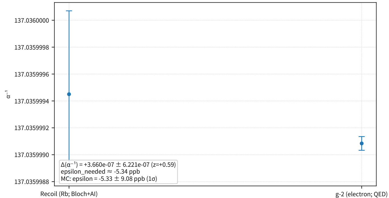
de Broglie precision cross-check via alpha (recoil vs electron g-2)
