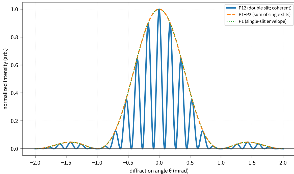
electron double-slit diffraction (600 eV; 50 nm slit, 280 nm sep.)
