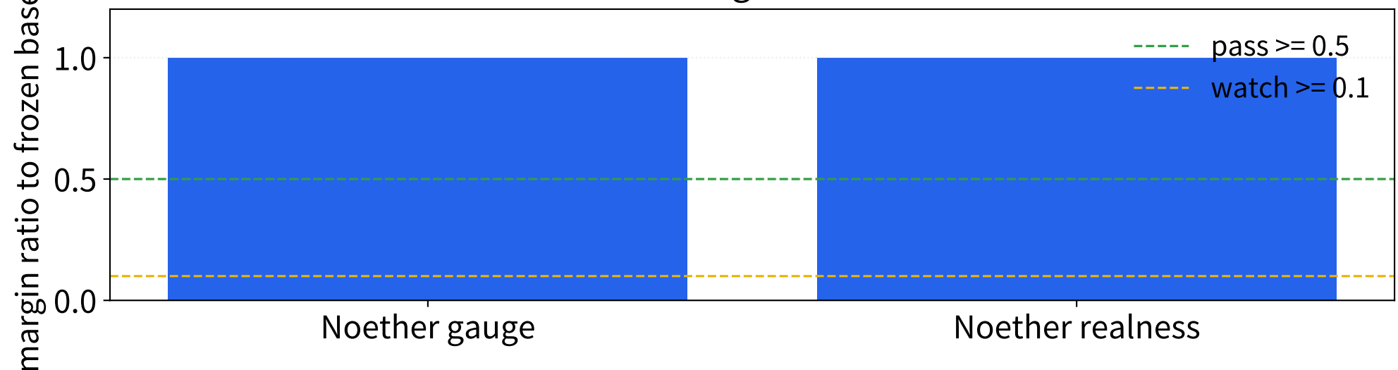
Noether margin-ratio watch
