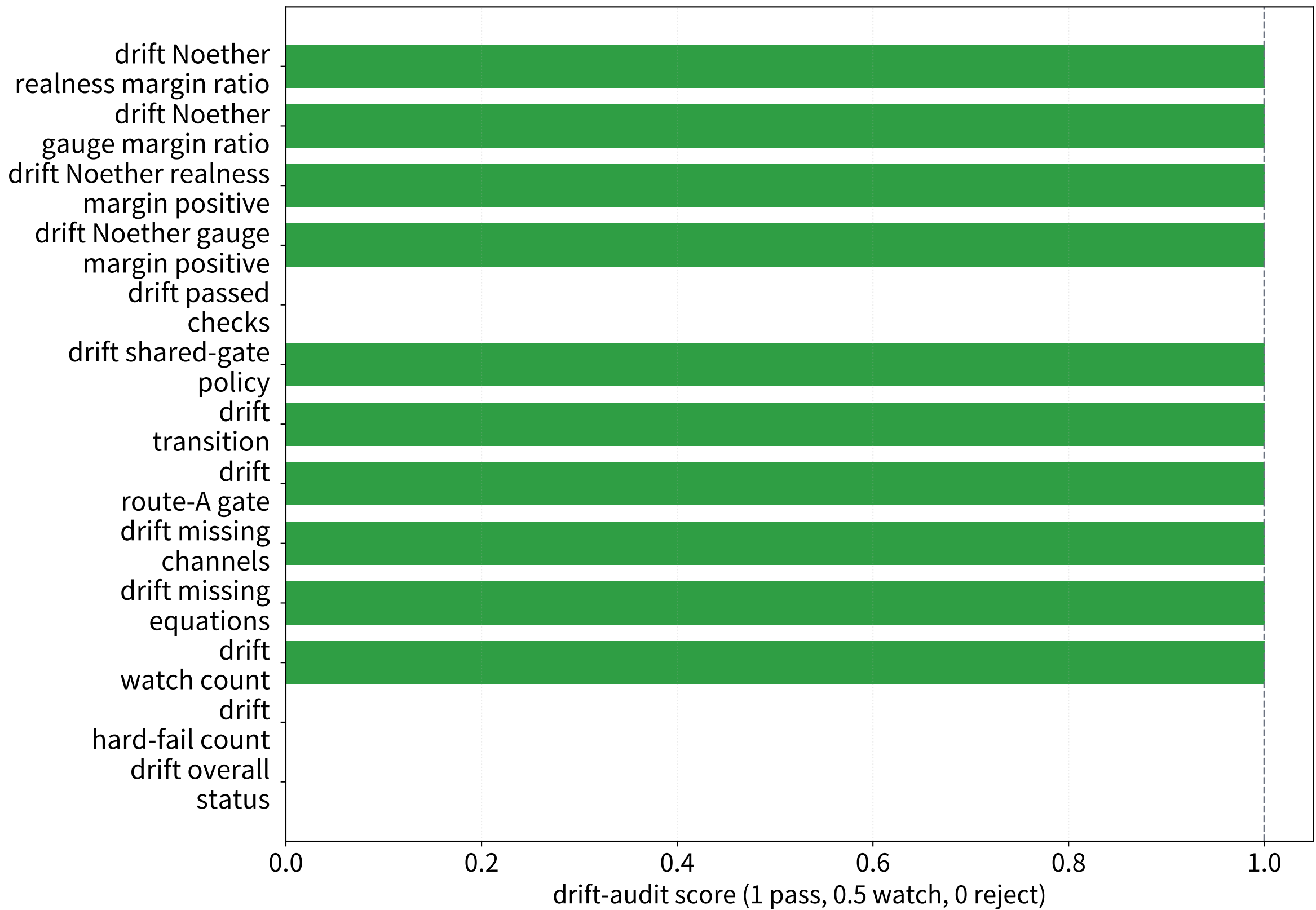
observable-closure drift audit
