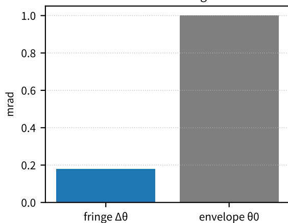
electron double-slit angular scale
