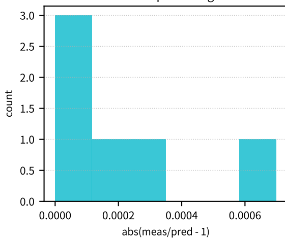
molecular isotopic scaling residual
