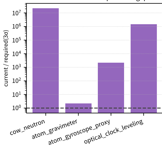
atom interferometer precision gap
