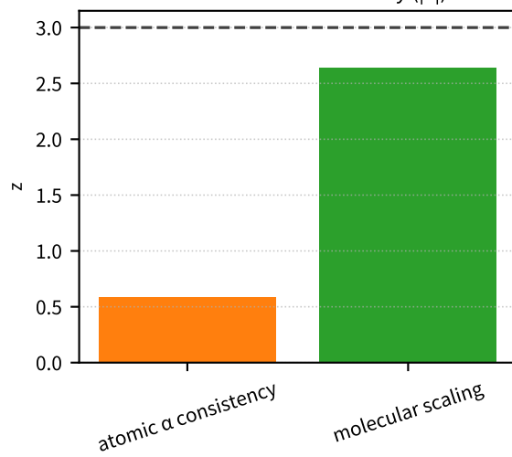
cross-channel consistency ( |z| )
