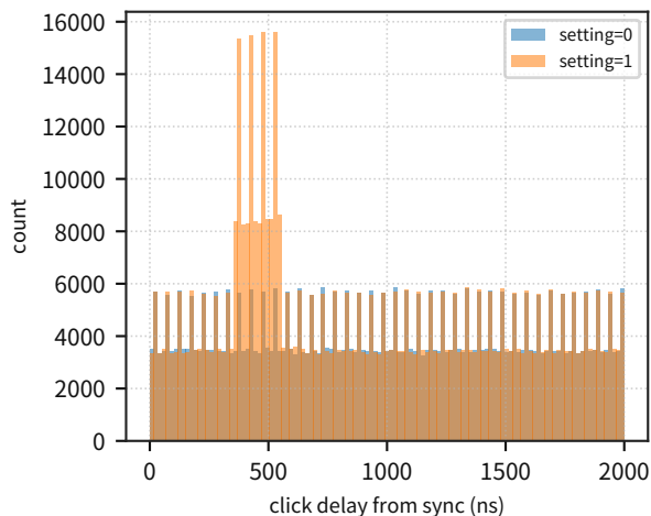
Alice: delay vs setting
