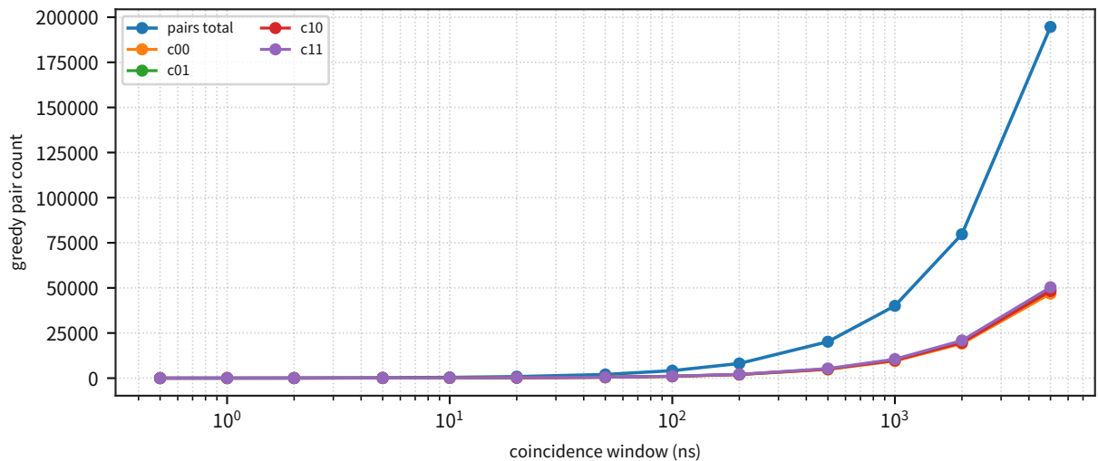
window dependence (GPS PPS alignment)
