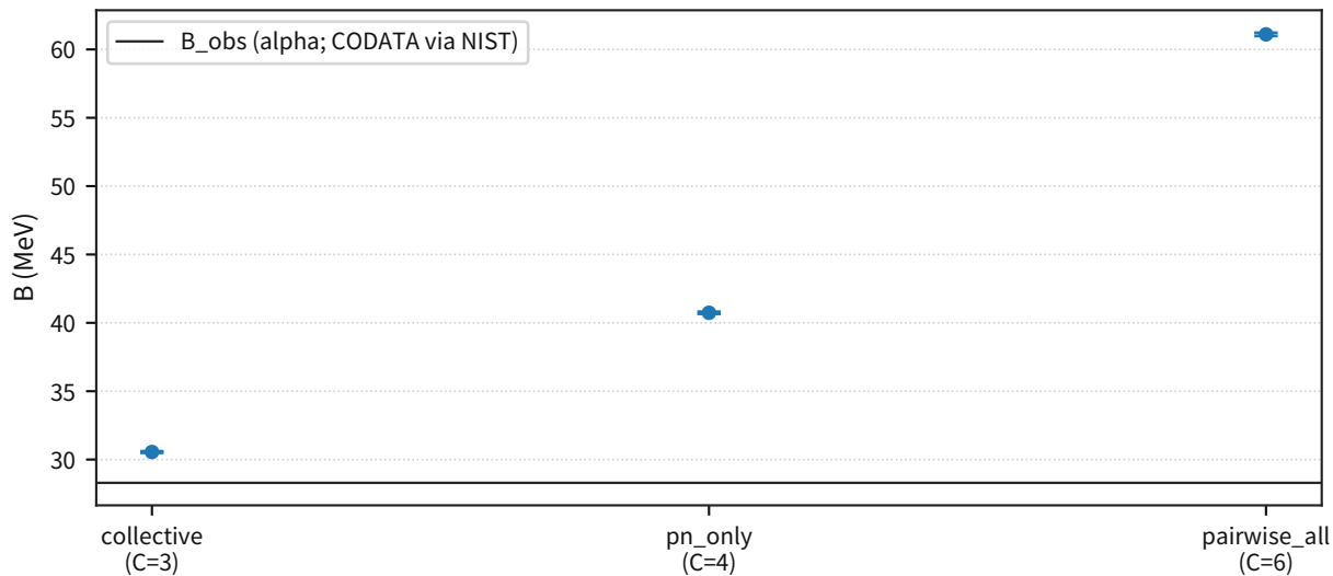
He-4 binding: multi-body reduction candidates
