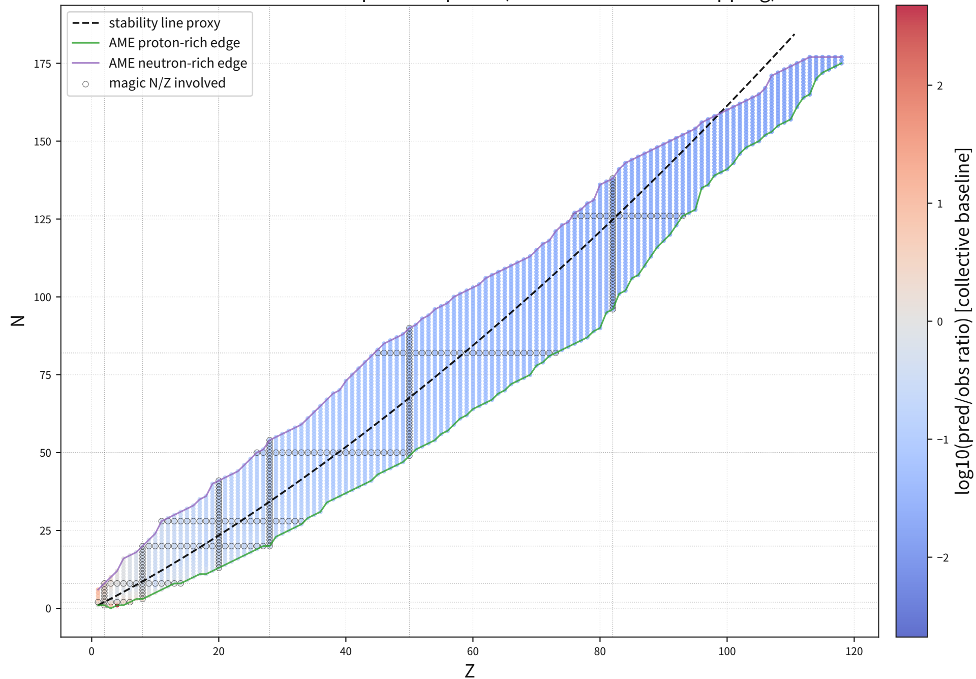
AME2020 residual map on Z-N plane (baseline collective mapping)
