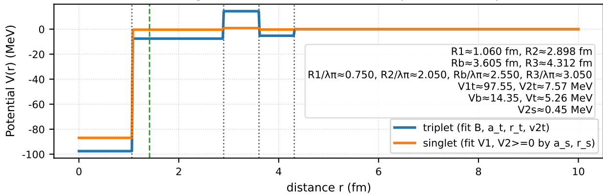
eq18 (GWU/SAID) three-range ( \lambda\pi constrained, barrier+tail split, free tail depth)
