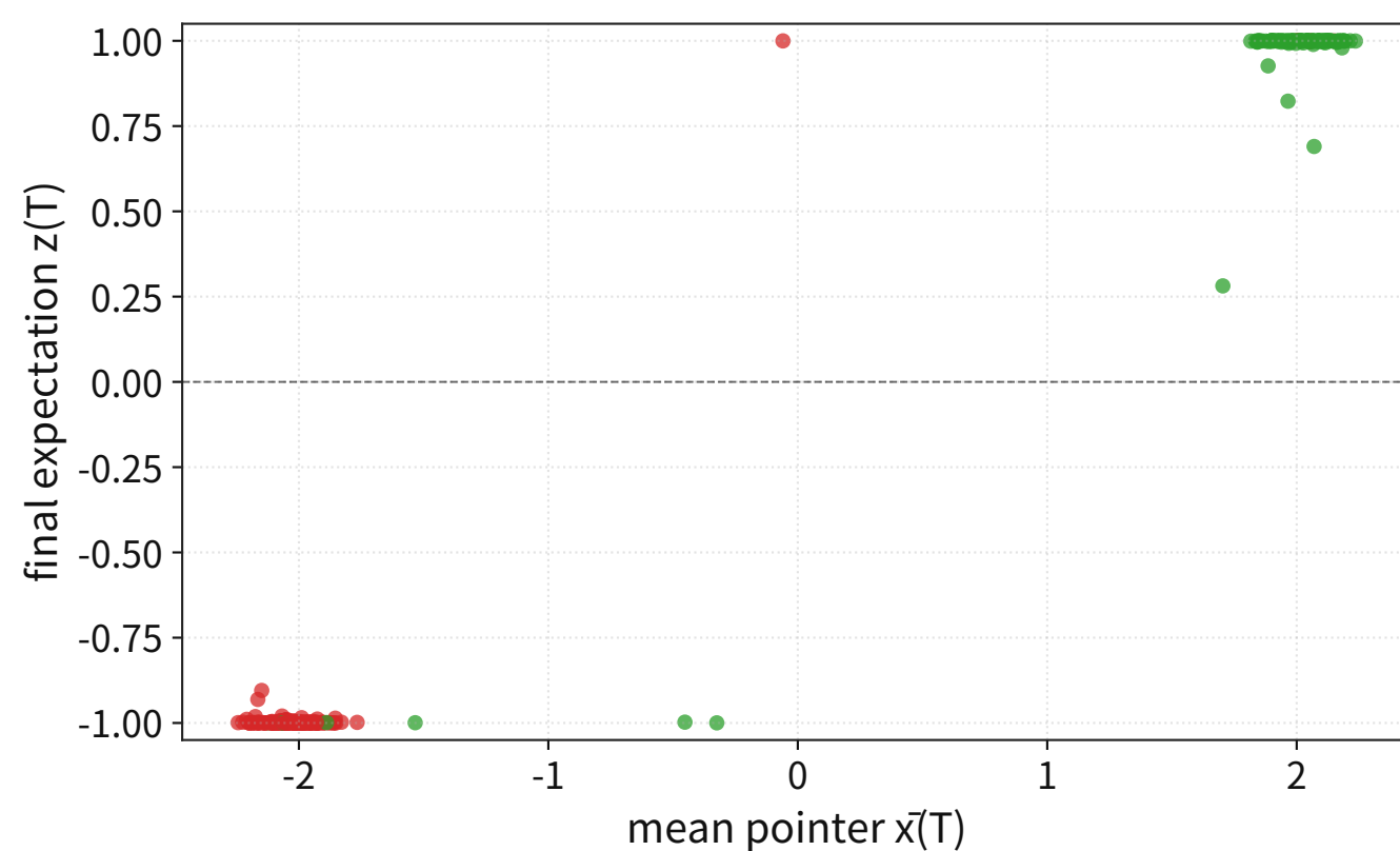
final-state scatter
