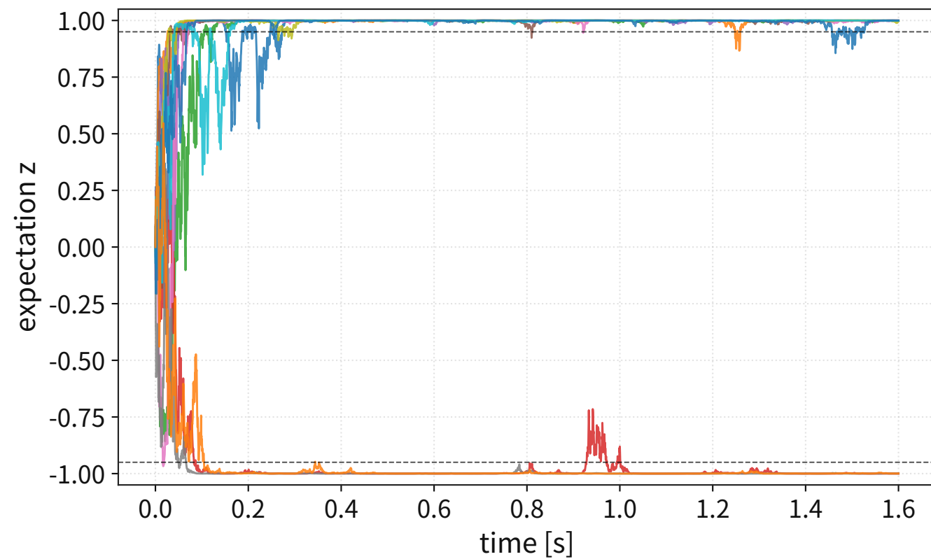
collapse-time distribution
