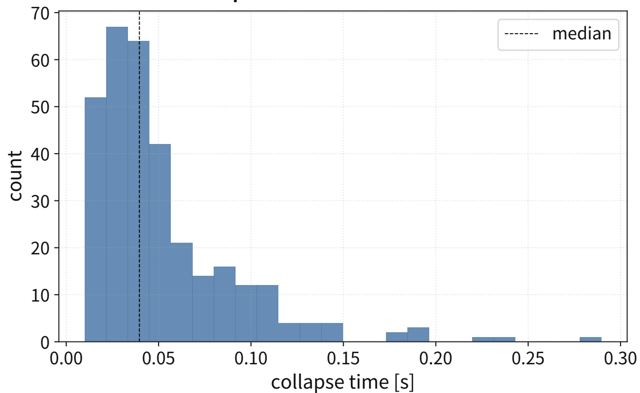
collapse-time distribution
