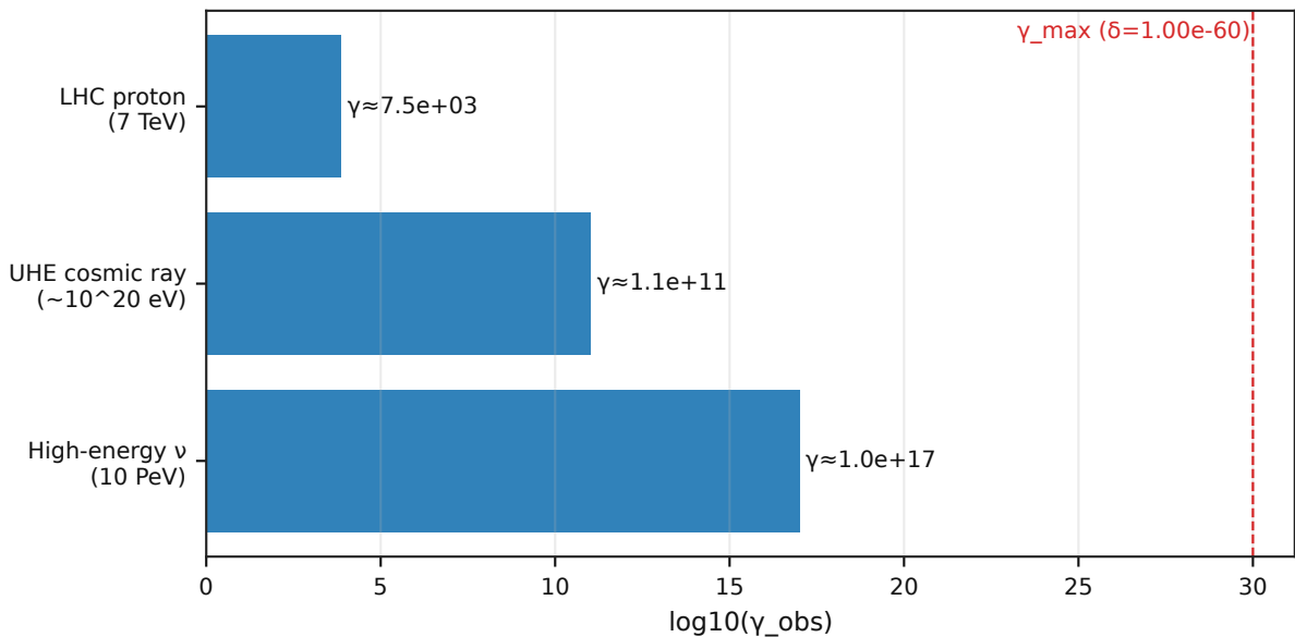
Observed Lorentz-factor scale
