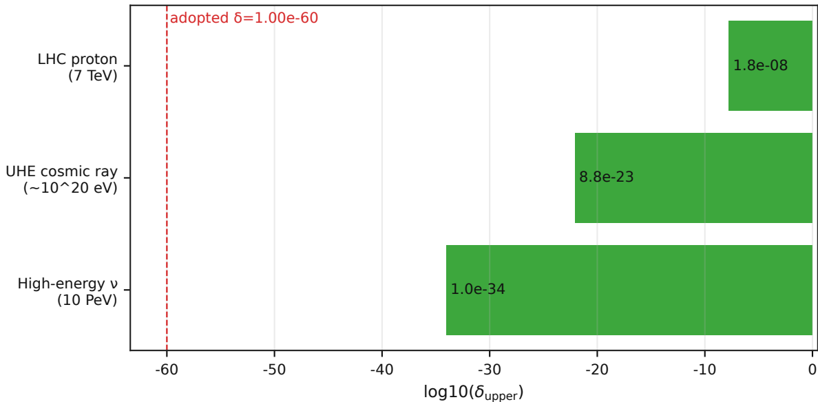
Approximate \delta upper bounds
