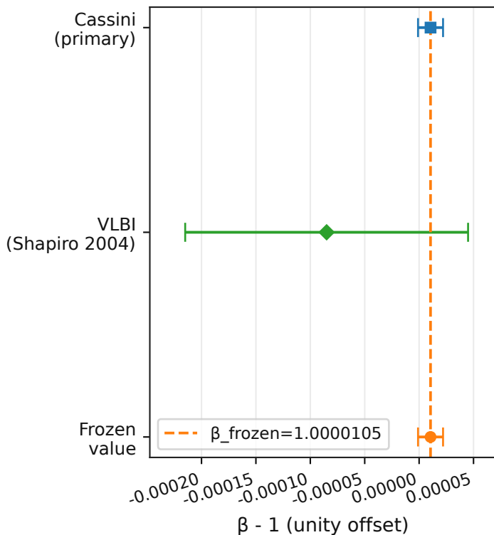
Left panel: \beta - 1
