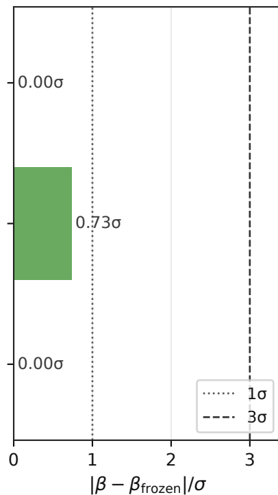
Right panel: |\beta - \beta_{\text{frozen}}|/\sigma
