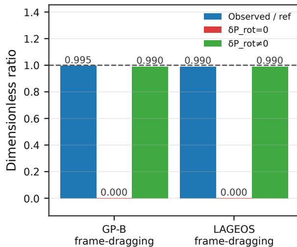
Frame-dragging ratio audit
