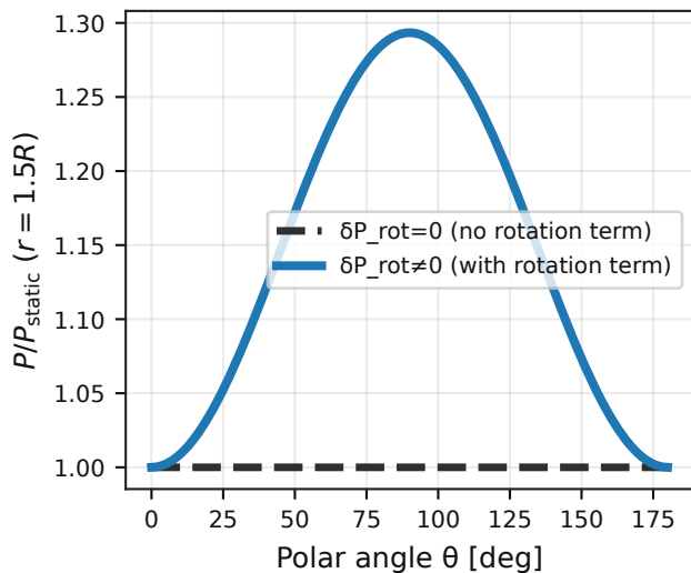
Rotating P profile audit
