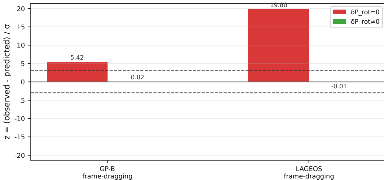
Precession gate comparison
