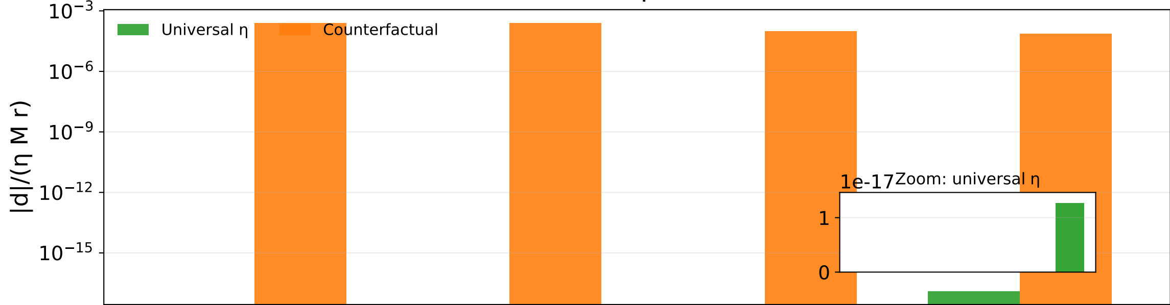
Normalized dipole moment
