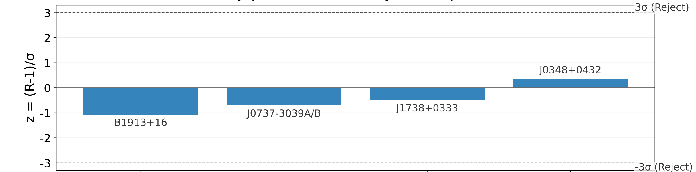
Binary-pulsar consistency with dipole = 0
