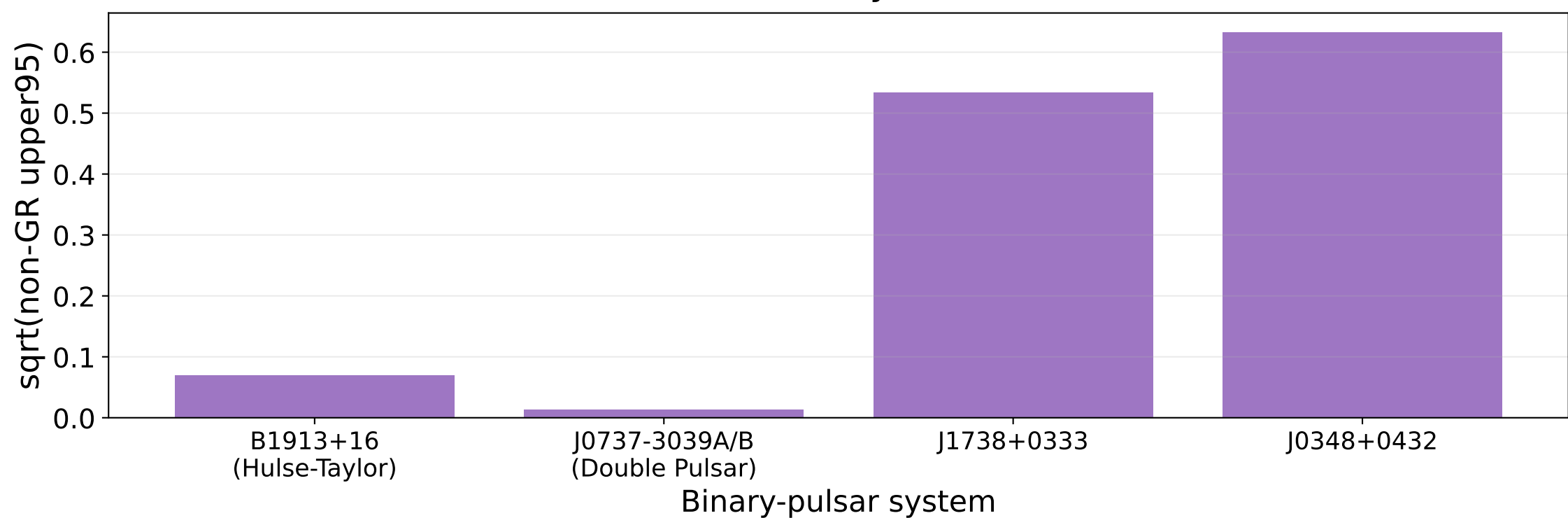
Estimated universality tolerance (95%)
