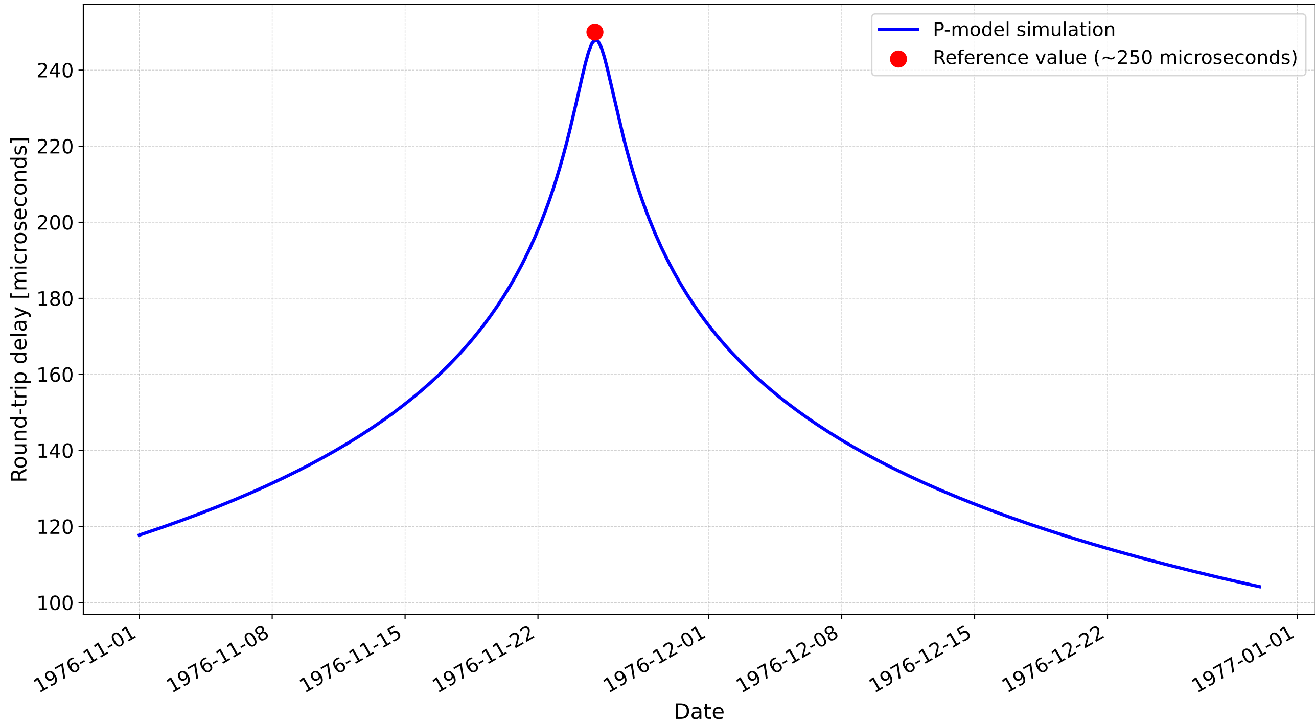
Viking solar conjunction (1976): P-model simulation vs reference value
