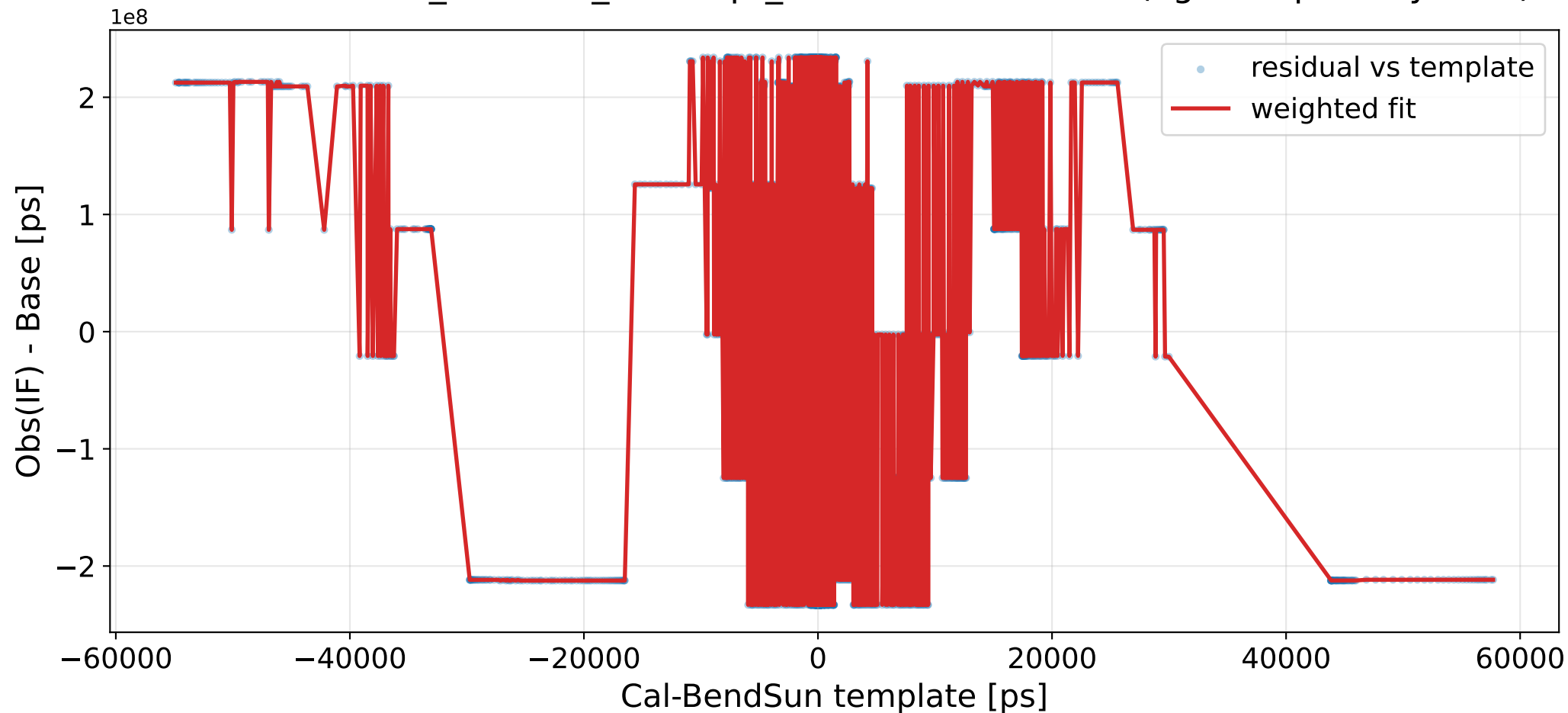
VLBI 17MAY01XA_baseline_intercept_linear direct beta fit (vgosDb primary data)
