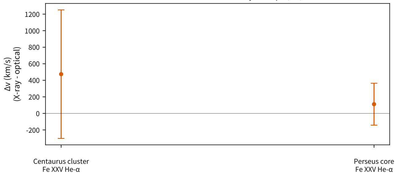
XRISM Resolve: cluster z_{\text{xray}} - z_{\text{opt}} ( \Delta v )
