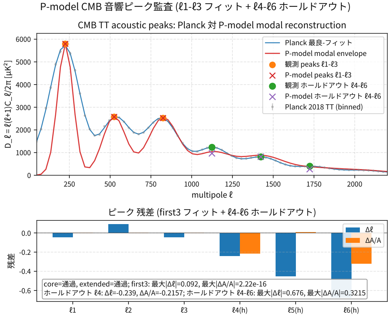
図 20: Comparison result for cosmology cmb acoustic peak reconstruction.
