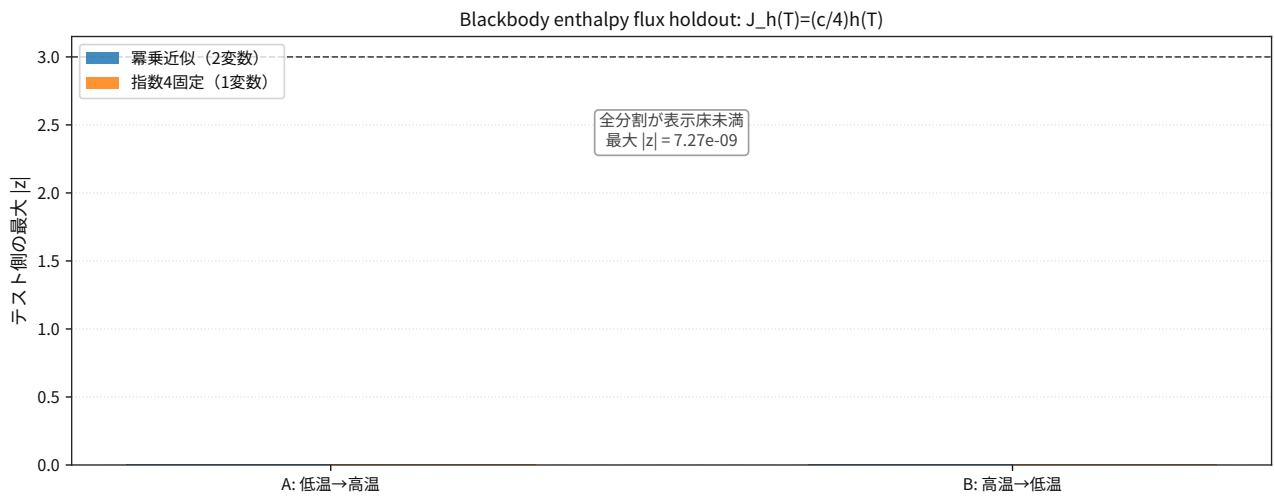
図 120: Comparison result for thermodynamics blackbody enthalpy flux holdout splits.
