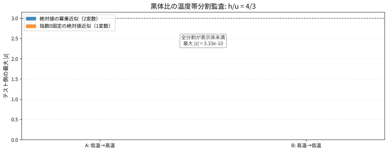
図 123: Comparison result for thermodynamics blackbody enthalpy energy ratio holdout splits.
