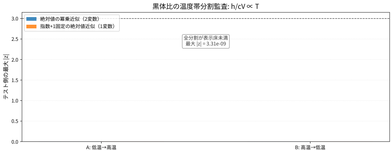
図 97: Comparison result for thermodynamics blackbody enthalpy per heat capacity density holdout splits.
