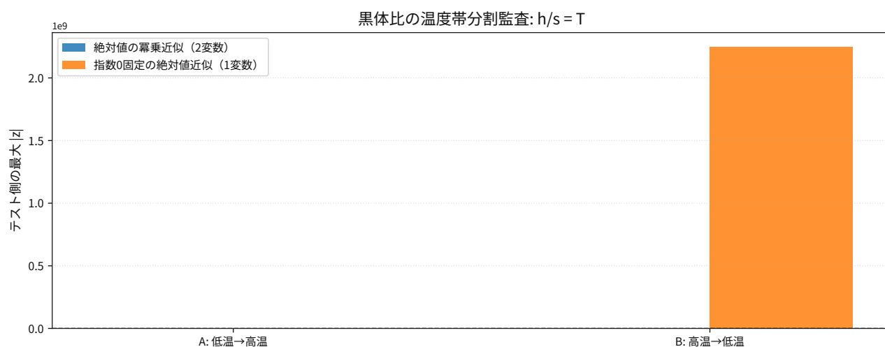
図 125: Comparison result for thermodynamics blackbody enthalpy entropy ratio holdout splits.
