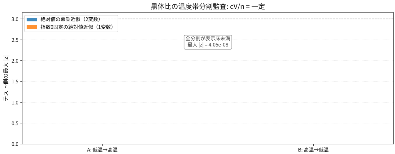
図 104: Comparison result for thermodynamics blackbody heat capacity per photon holdout splits.
