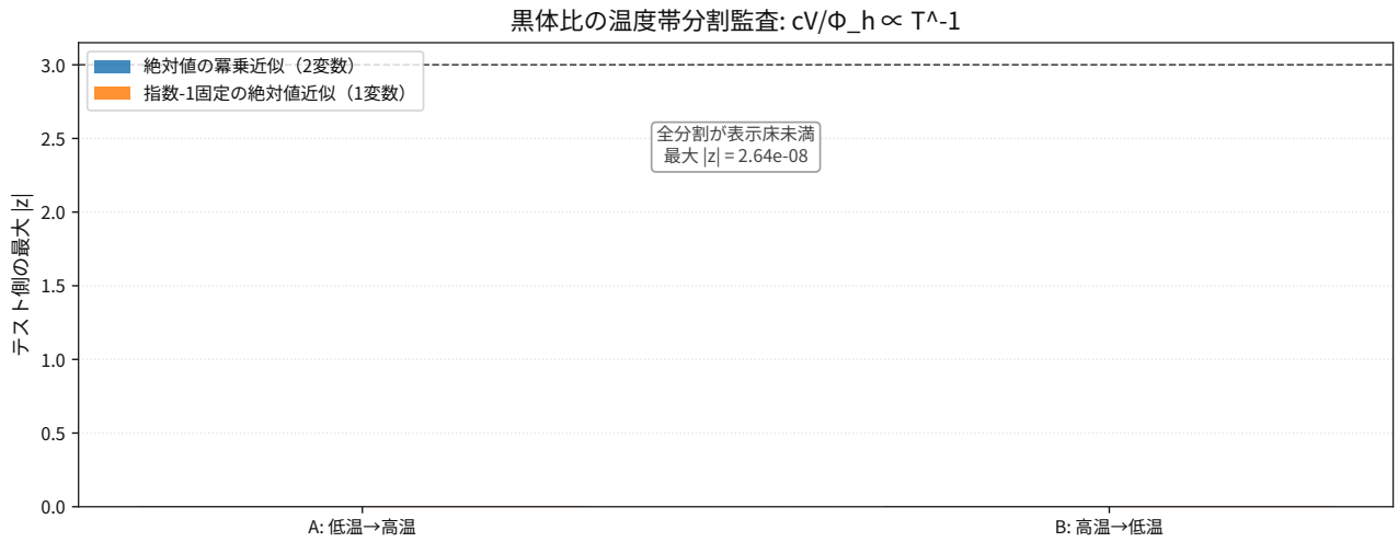
図 92: Comparison result for thermodynamics blackbody heat capacity per enthalpy flux holdout splits.
