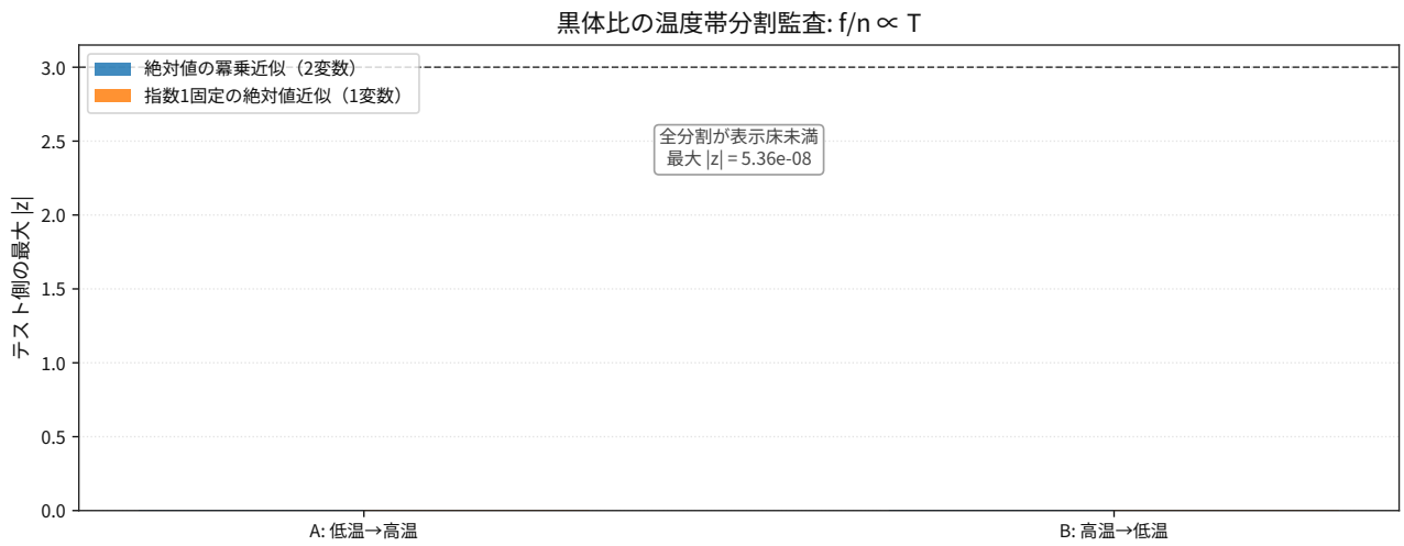
図 116: Comparison result for thermodynamics blackbody Helmholtz per photon holdout splits.
