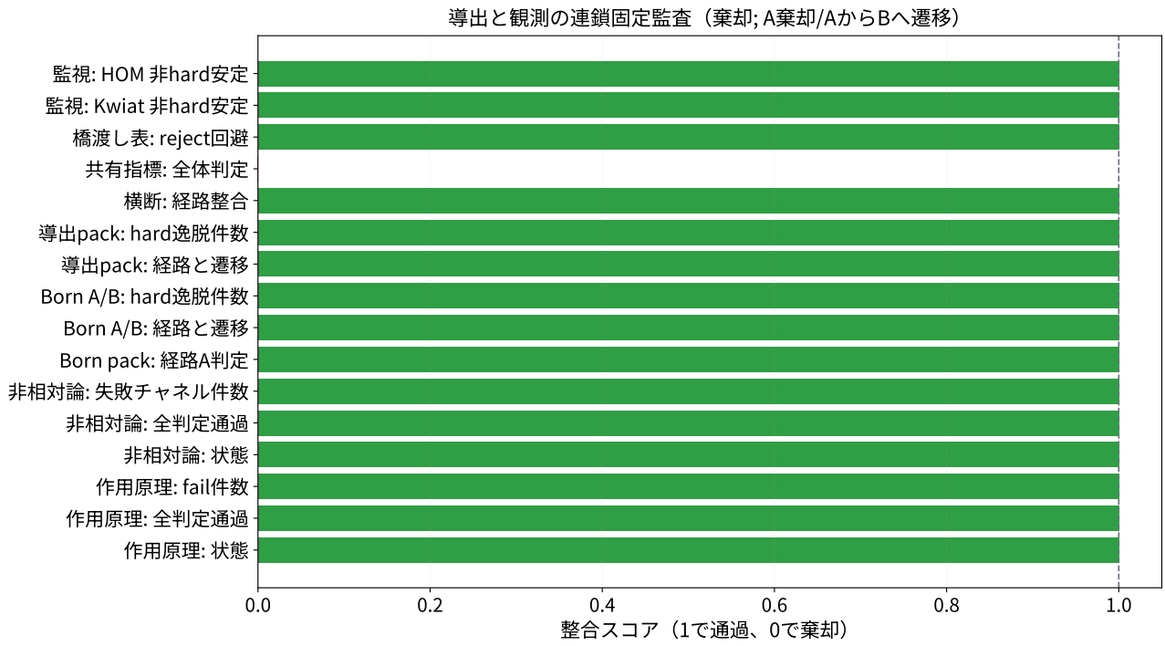
図 42: Comparison result for derivation observable chain lock audit.
