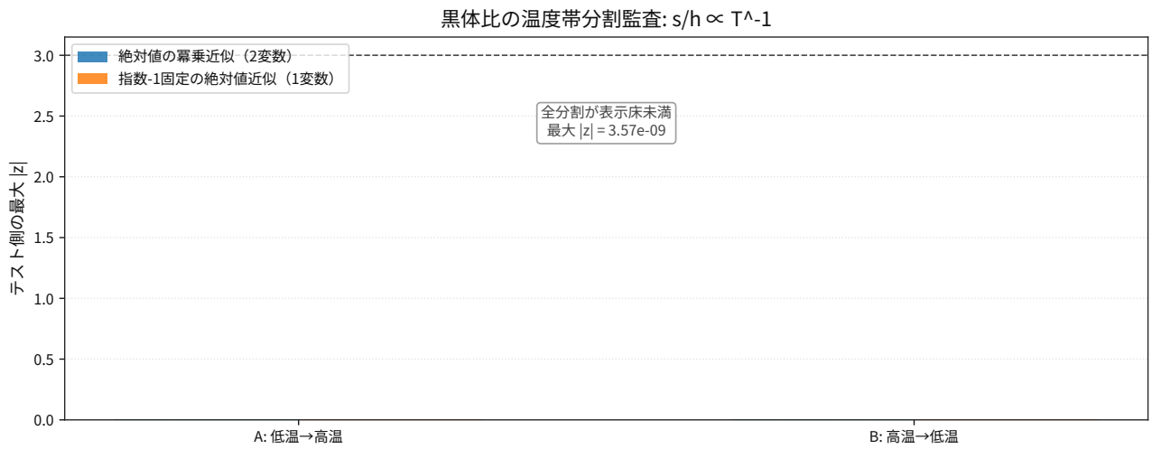
図 90: Comparison result for thermodynamics blackbody entropy per enthalpy density holdout splits.
