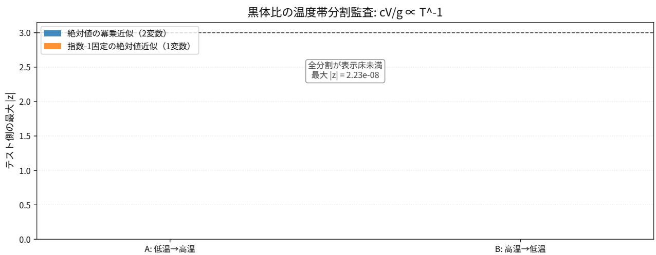
図 109: Comparison result for thermodynamics blackbody heat capacity momentum ratio holdout splits.
