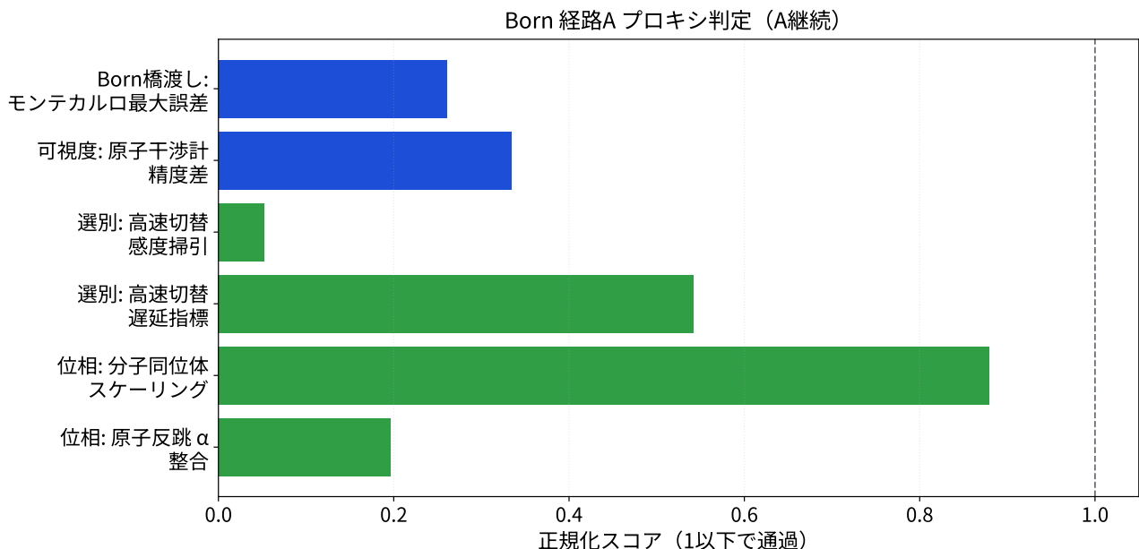
図 38: Comparison result for born route A proxy constraints pack.
