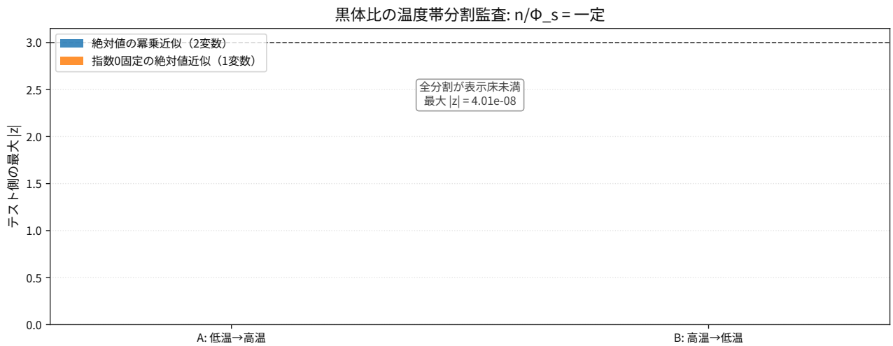
図 87: Comparison result for thermodynamics blackbody photon density per entropy flux holdout splits.
