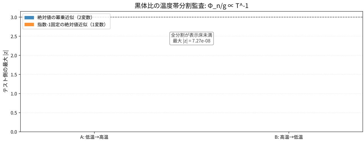
図 82: Comparison result for thermodynamics blackbody photon flux per momentum density holdout splits.
