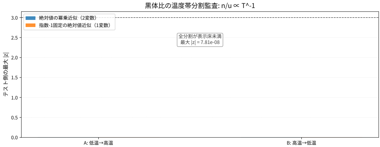
図 72: Comparison result for thermodynamics blackbody photon density per energy density holdout splits.
