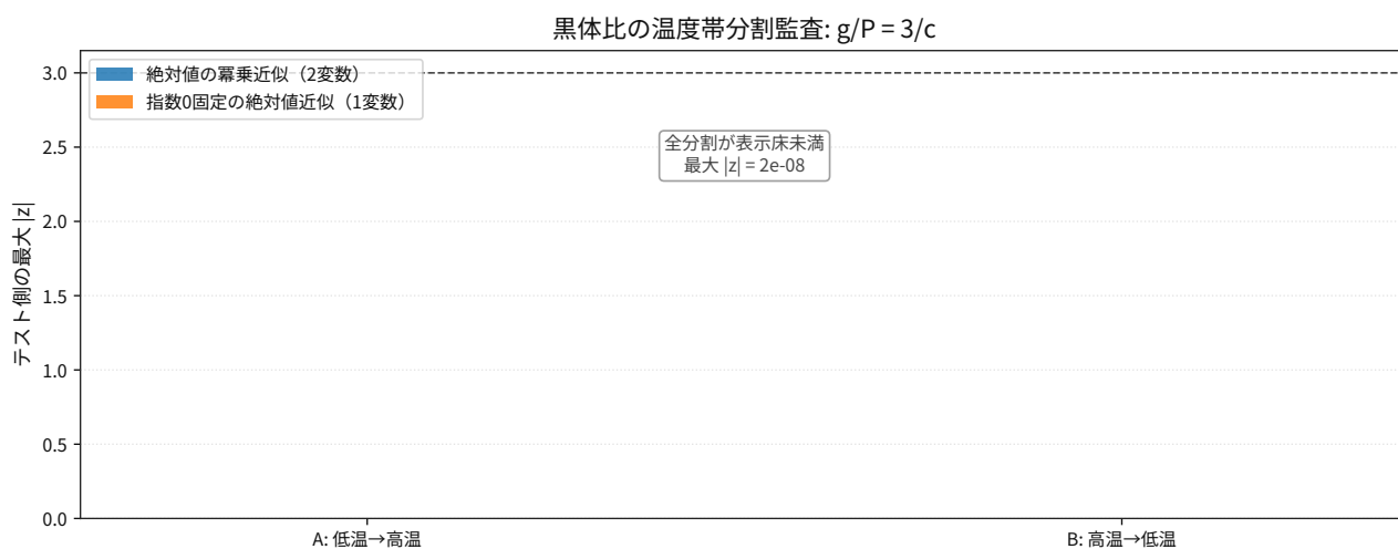
図 65: Comparison result for thermodynamics blackbody momentum pressure ratio holdout splits.
