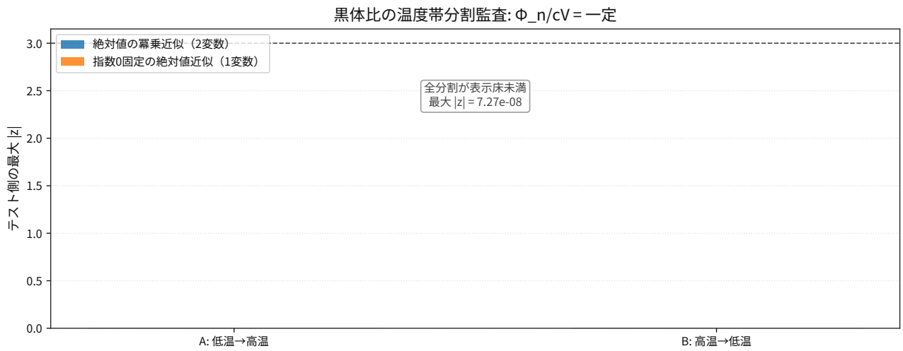
図 78: Comparison result for thermodynamics blackbody photon flux per heat capacity density holdout splits.
