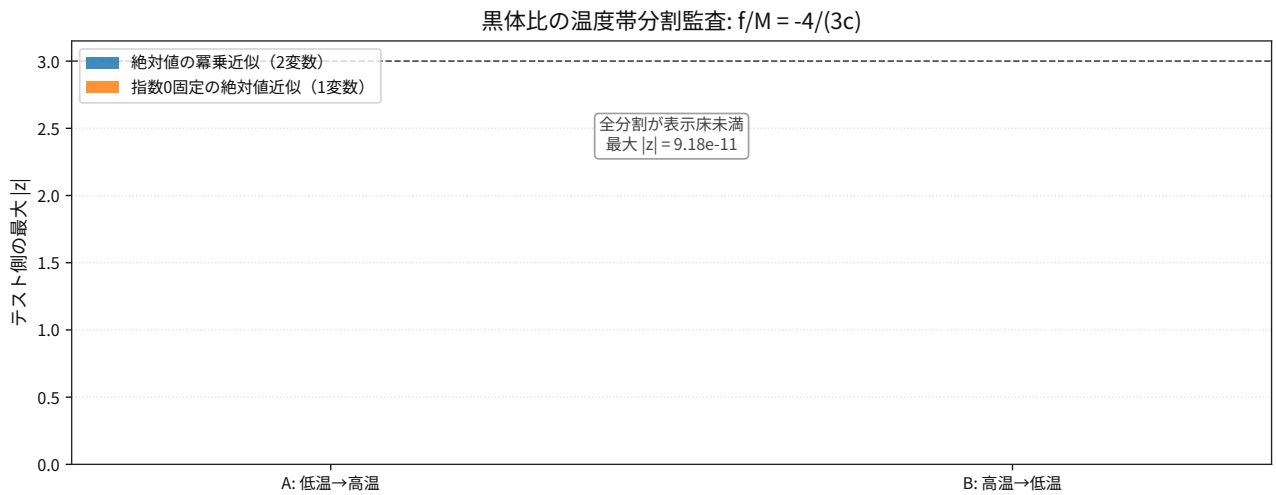
図 135: Comparison result for thermodynamics blackbody Helmholtz flux ratio holdout splits.
