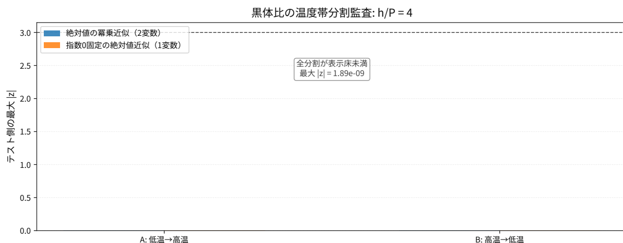
図 124: Comparison result for thermodynamics blackbody enthalpy pressure ratio holdout splits.
