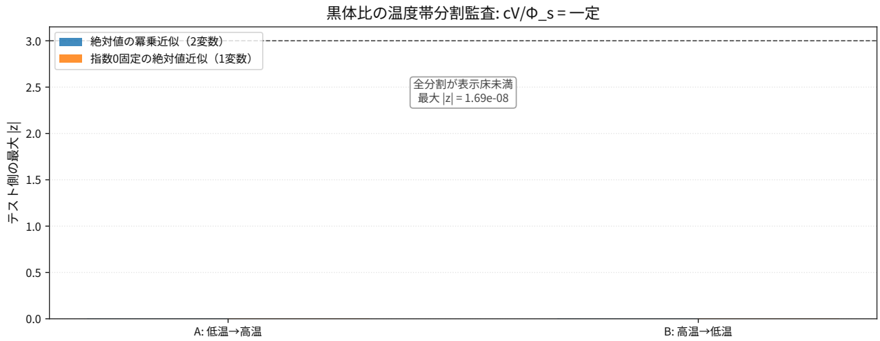
図 106: Comparison result for thermodynamics blackbody heat capacity per entropy flux holdout splits.
