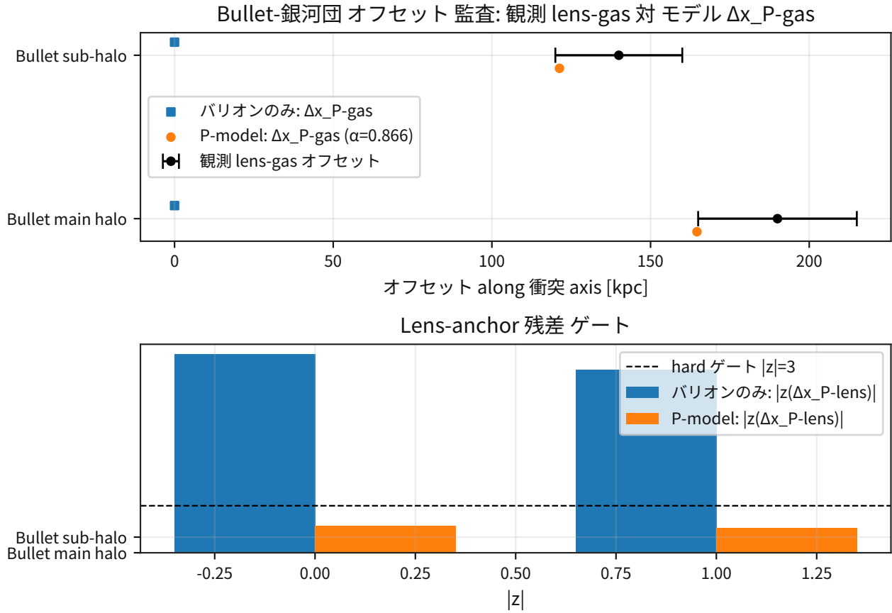
図 9: Comparison result for cosmology cluster collision p peak offset audit.
