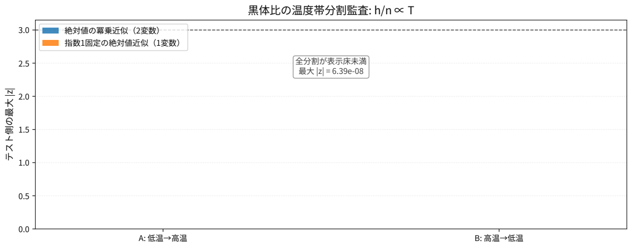
図 113: Comparison result for thermodynamics blackbody enthalpy per photon holdout splits.
