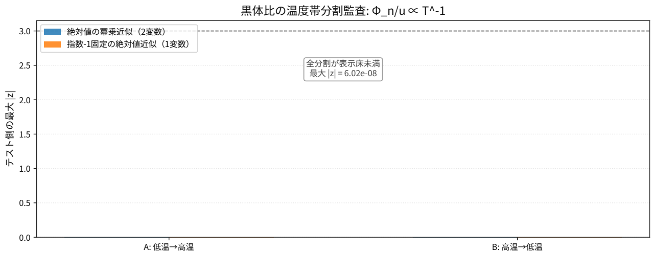
図 75: Comparison result for thermodynamics blackbody photon flux per energy density holdout splits.
