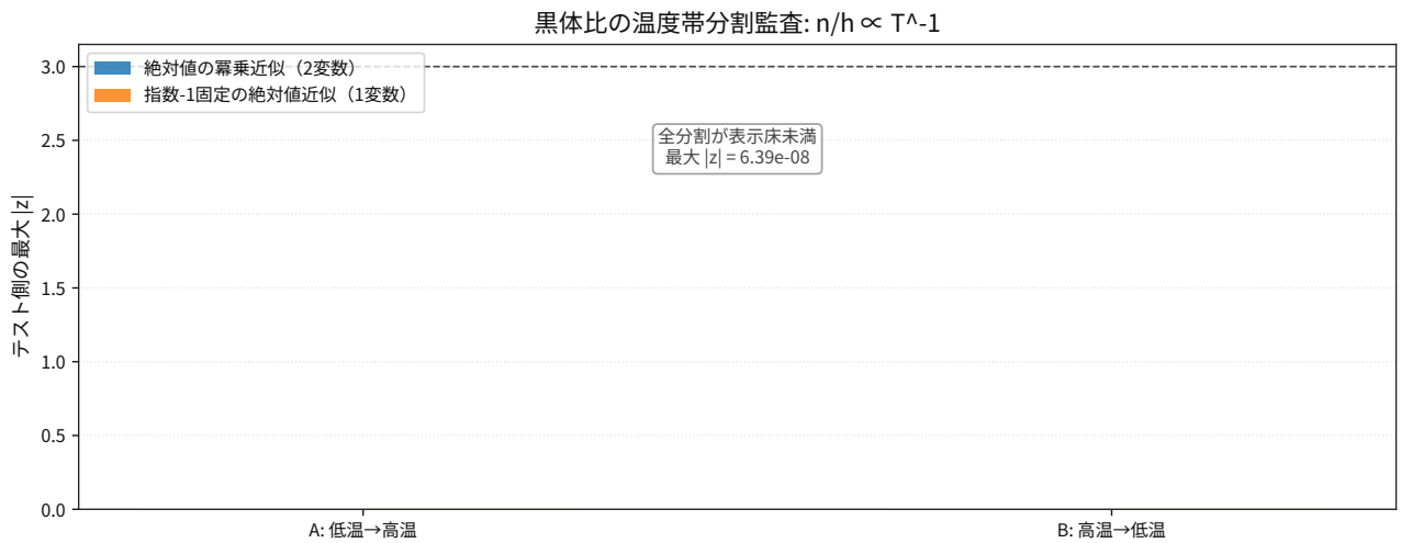
図 73: Comparison result for thermodynamics blackbody photon density per enthalpy density holdout splits.
