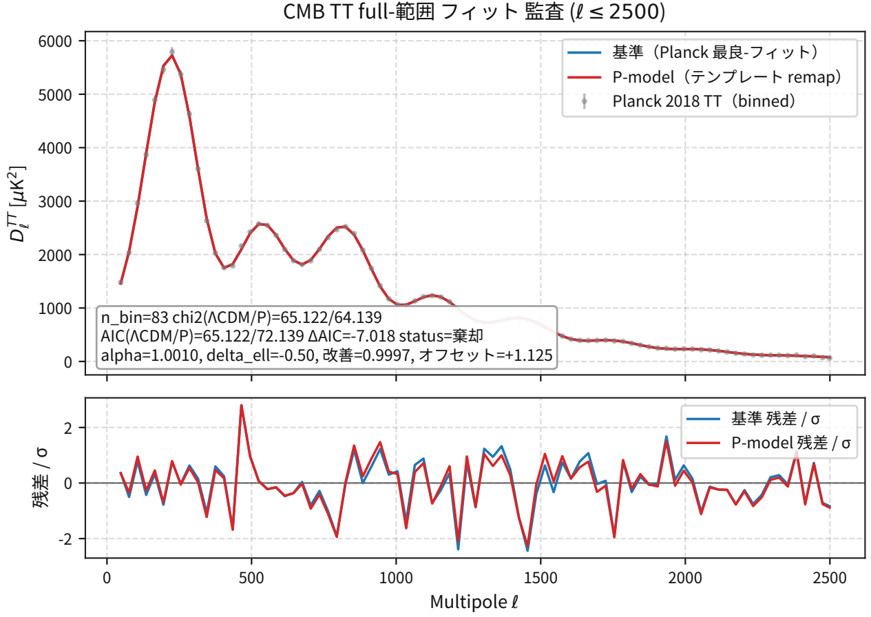
図 21: Comparison result for cosmology cmb tt full cl fit.
