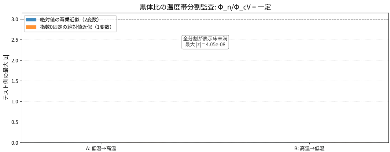
図 79: Comparison result for thermodynamics blackbody photon flux per heat capacity flux holdout splits.
