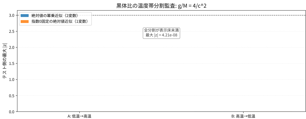
図 133: Comparison result for thermodynamics blackbody momentum flux ratio holdout splits.
