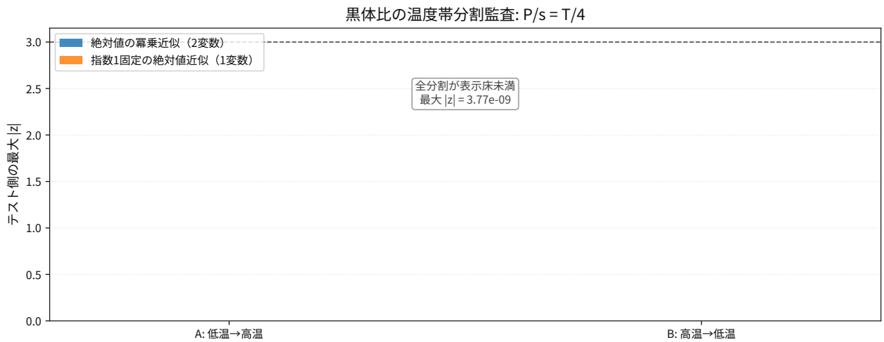
図 131: Comparison result for thermodynamics blackbody pressure entropy ratio holdout splits.
