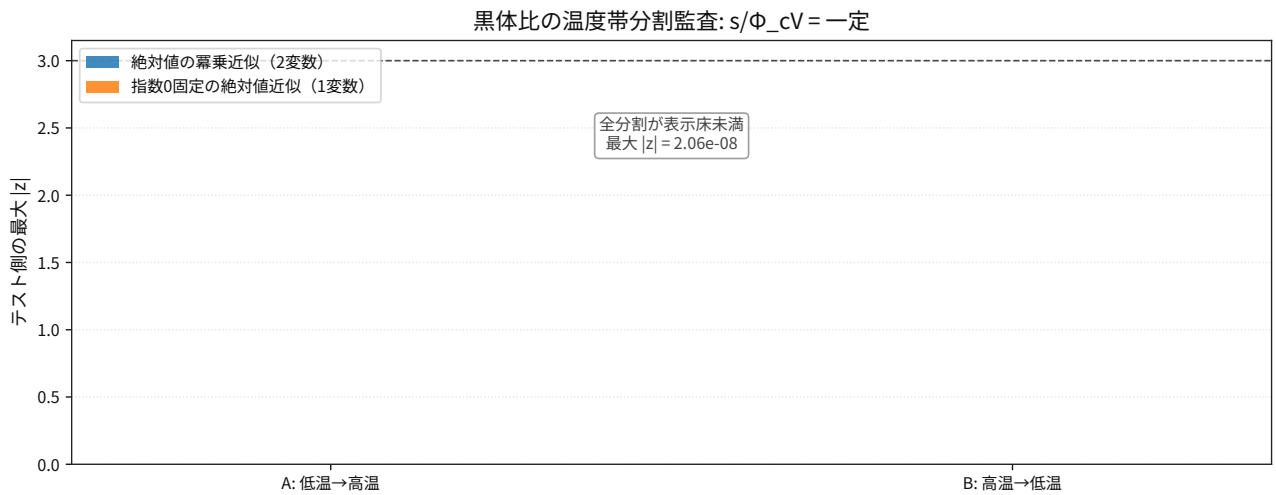
図 101: Comparison result for thermodynamics blackbody entropy per heat capacity flux holdout splits.
