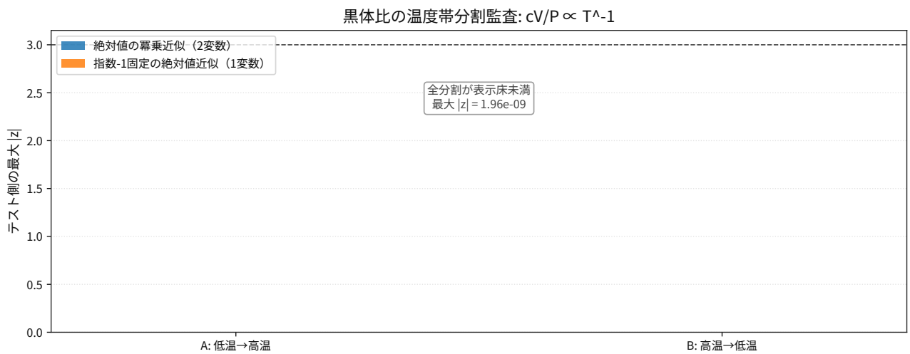
図 111: Comparison result for thermodynamics blackbody heat capacity pressure ratio holdout splits.
