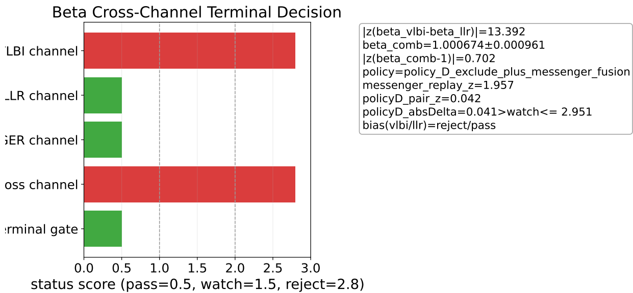
図 15: Comparison result for beta cross channel registry.
