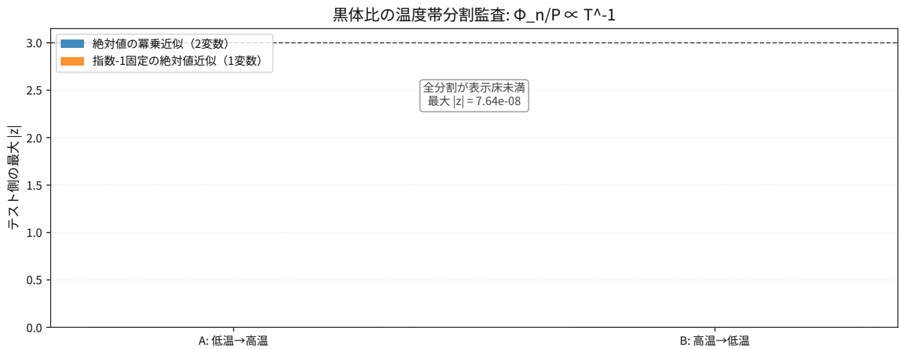
図 77: Comparison result for thermodynamics blackbody photon flux per pressure holdout splits.
