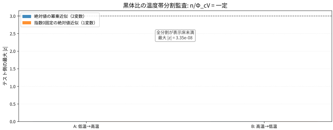
図 102: Comparison result for thermodynamics blackbody photon density per heat capacity flux holdout splits.
