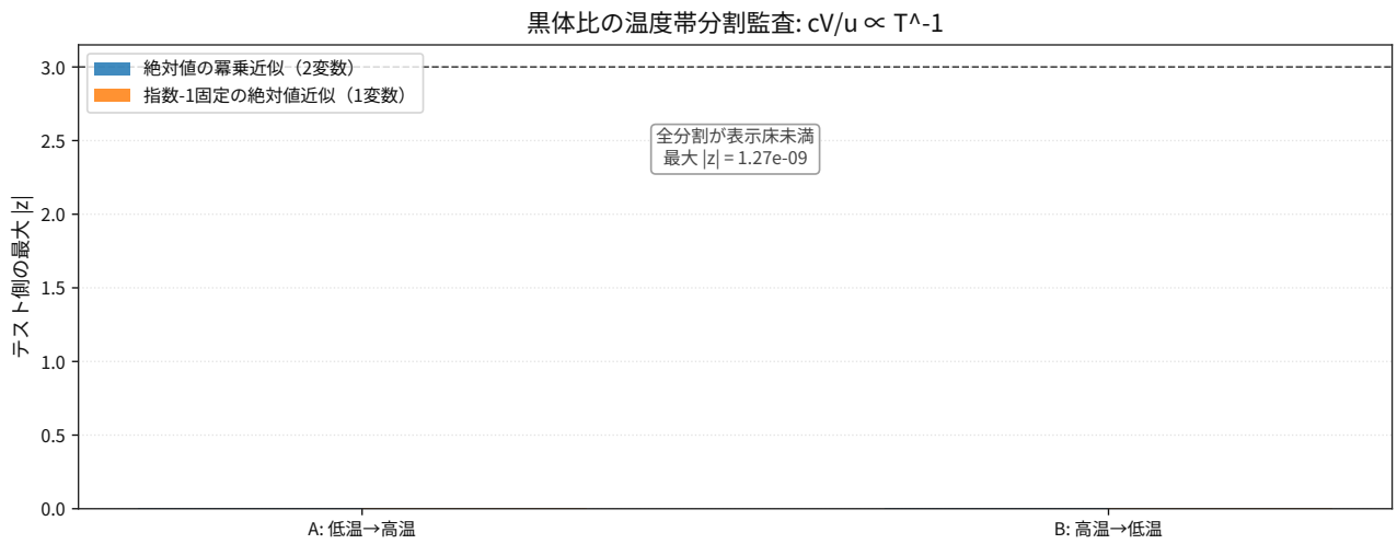
図 110: Comparison result for thermodynamics blackbody heat capacity energy ratio holdout splits.
