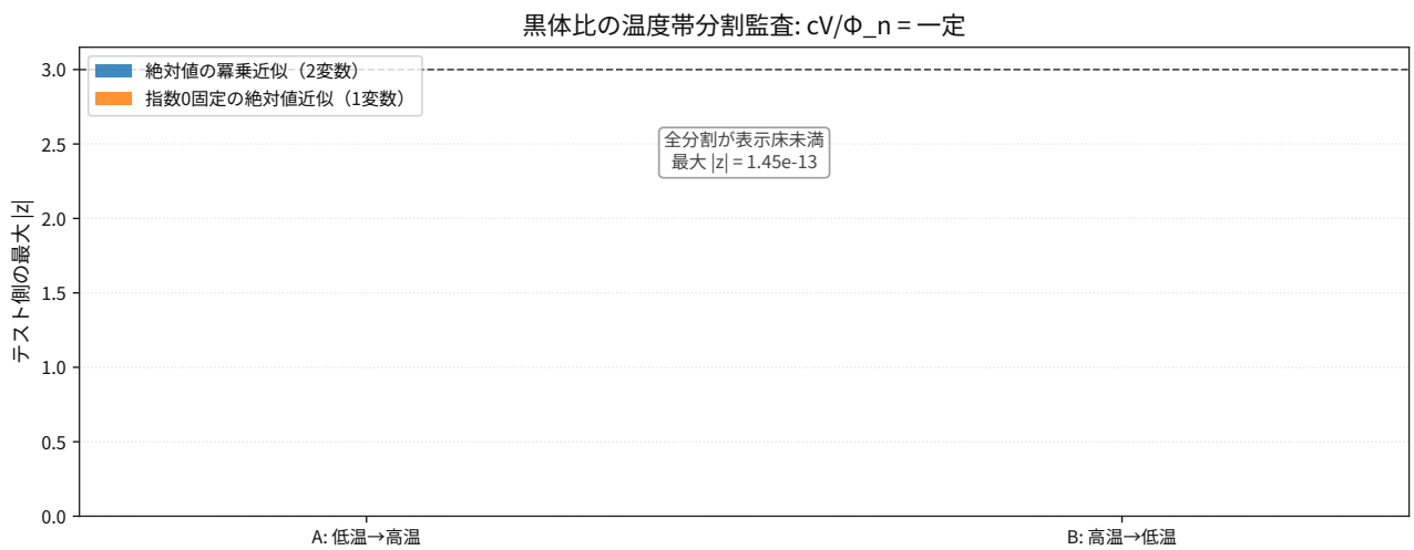
図 105: Comparison result for thermodynamics blackbody heat capacity per photon flux holdout splits.
