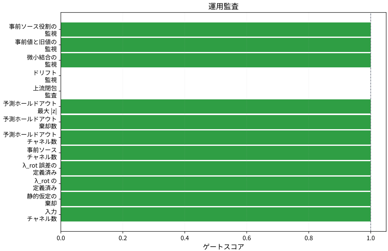
図 45: Comparison result for lagrangian noether rotational closure audit.
