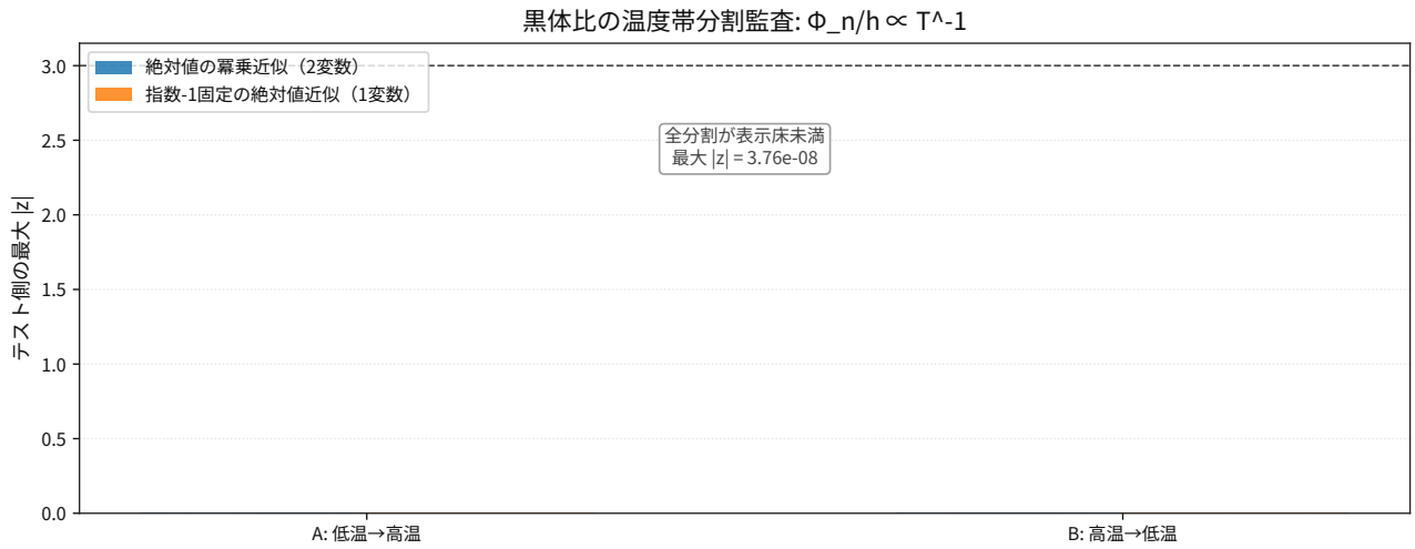
図 76: Comparison result for thermodynamics blackbody photon flux per enthalpy density holdout splits.
