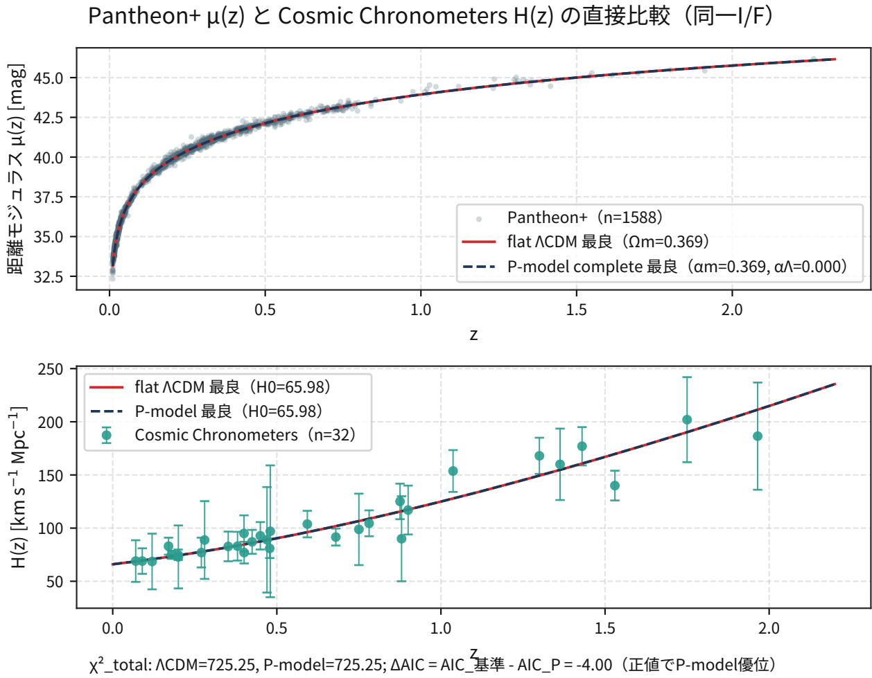
図 19: Comparison result for cosmology pantheonplus cc direct fit.
