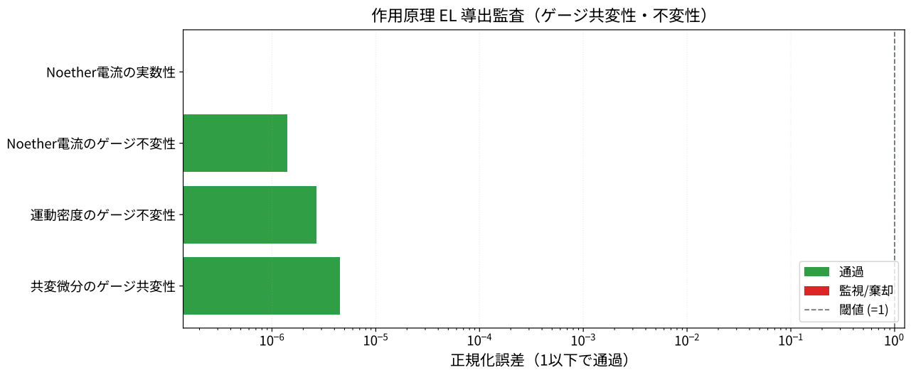
図 39: Comparison result for action principle EL derivation audit.
