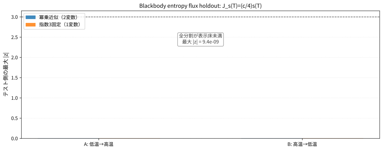
図 119: Comparison result for thermodynamics blackbody entropy flux holdout splits.
