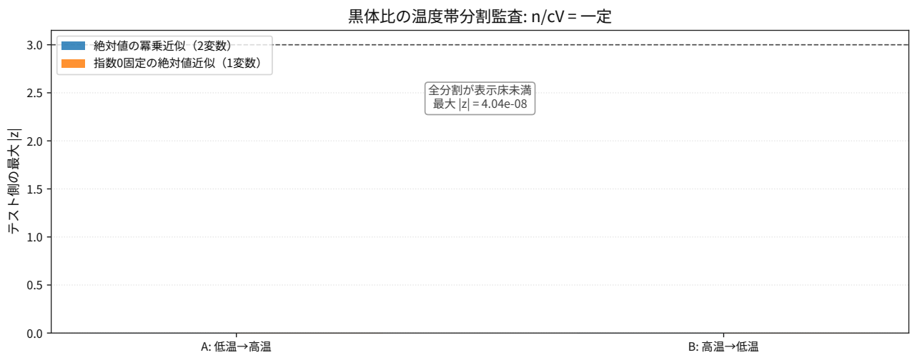
図 103: Comparison result for thermodynamics blackbody photon density per heat capacity density holdout splits.
