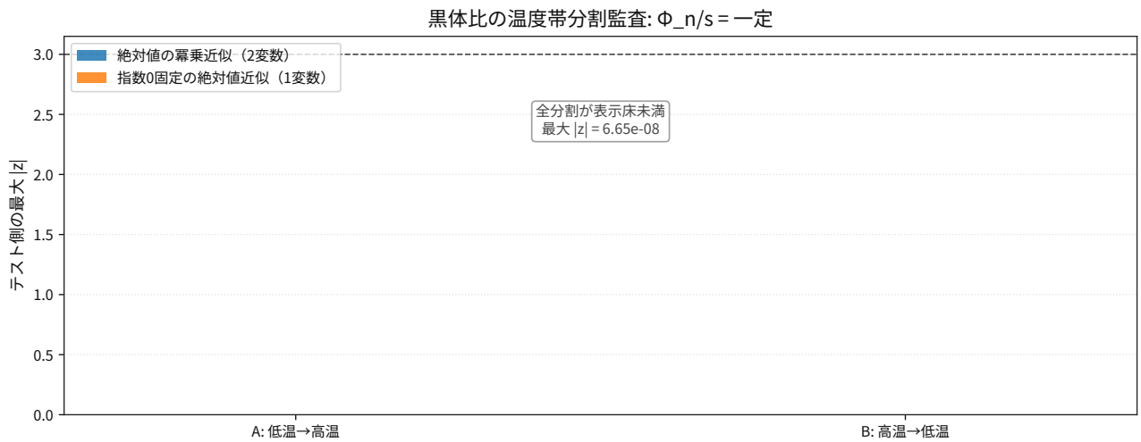
図 81: Comparison result for thermodynamics blackbody photon flux per entropy density holdout splits.
