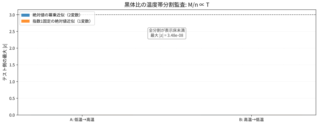
図 118: Comparison result for thermodynamics blackbody flux per photon holdout splits.
