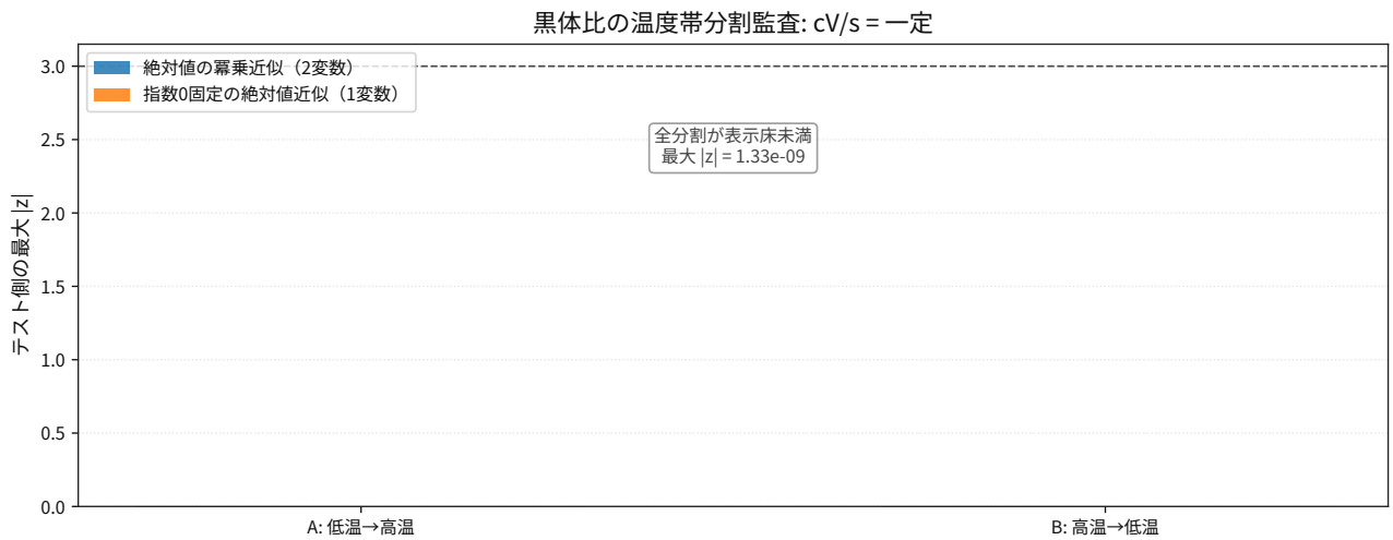
図 107: Comparison result for thermodynamics blackbody heat capacity entropy ratio holdout splits.
