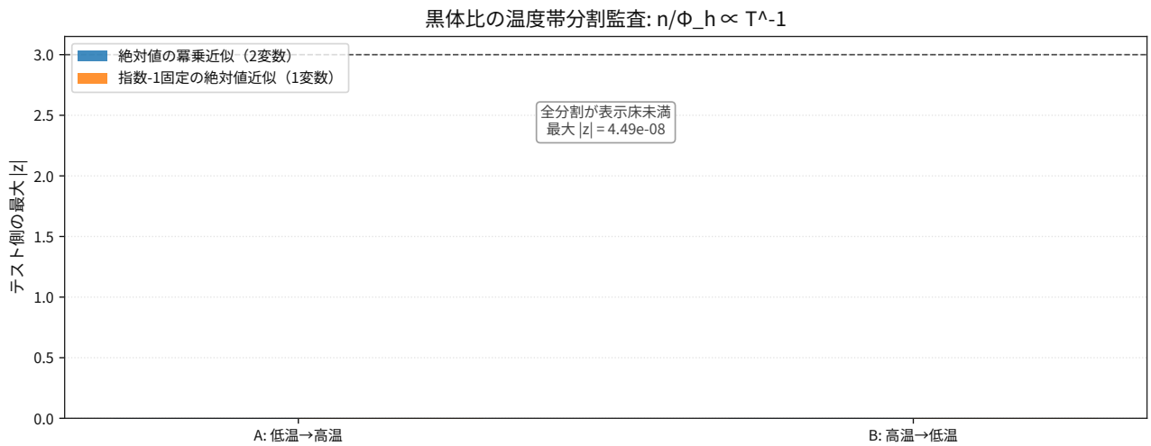
図 93: Comparison result for thermodynamics blackbody photon density per enthalpy flux holdout splits.
