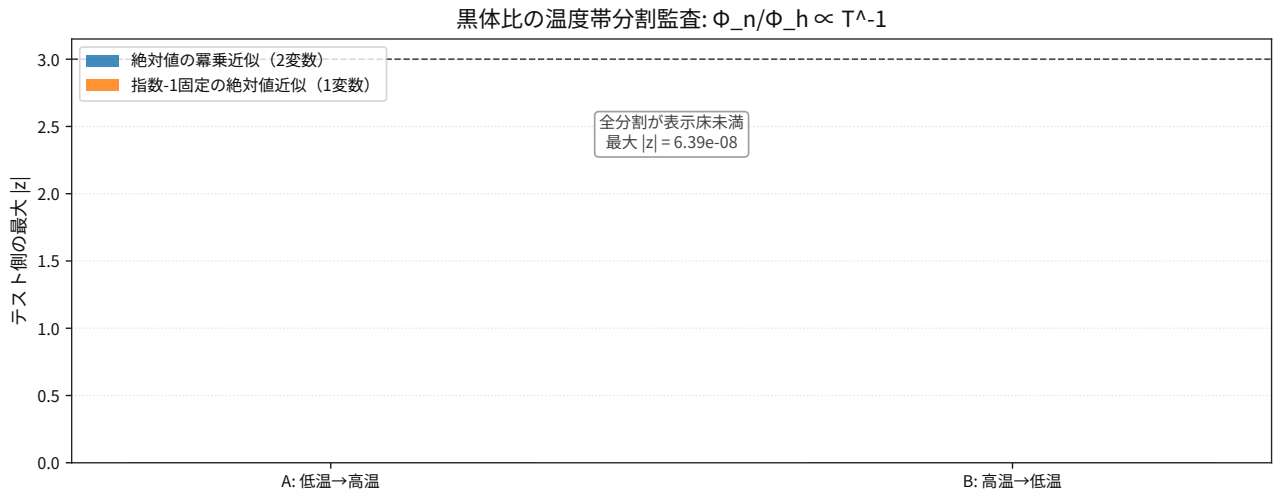
図 80: Comparison result for thermodynamics blackbody photon flux per enthalpy flux holdout splits.
