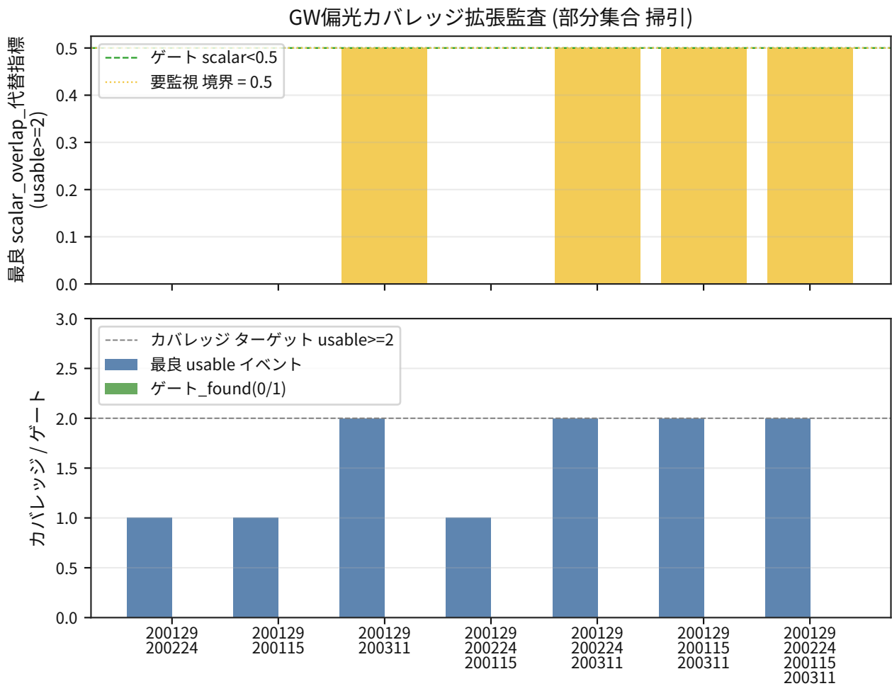
図 32: Comparison result for GW polarization network coverage expansion audit.
