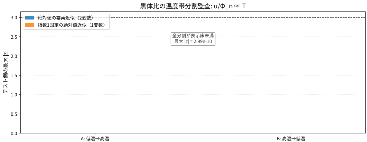
図 115: Comparison result for thermodynamics blackbody energy per photon flux holdout splits.
