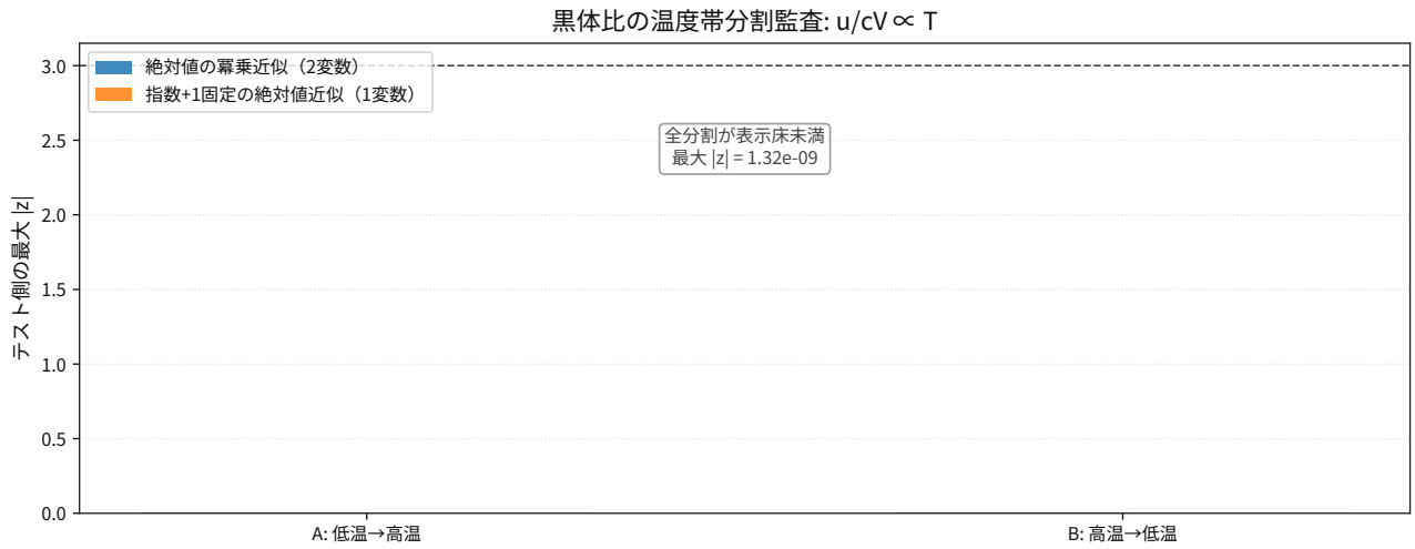
図 96: Comparison result for thermodynamics blackbody energy per heat capacity density holdout splits.
