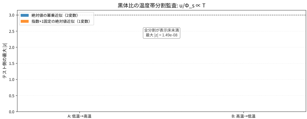
図 85: Comparison result for thermodynamics blackbody energy per entropy flux holdout splits.
