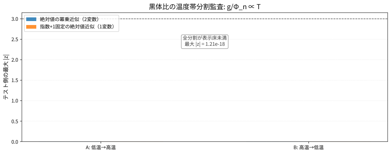
図 69: Comparison result for thermodynamics blackbody momentum per photon flux holdout splits.
