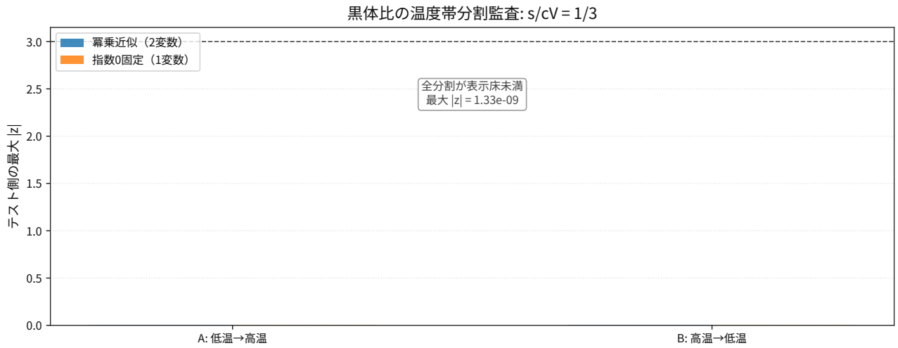
図 98: Comparison result for thermodynamics blackbody entropy per heat capacity density holdout splits.
