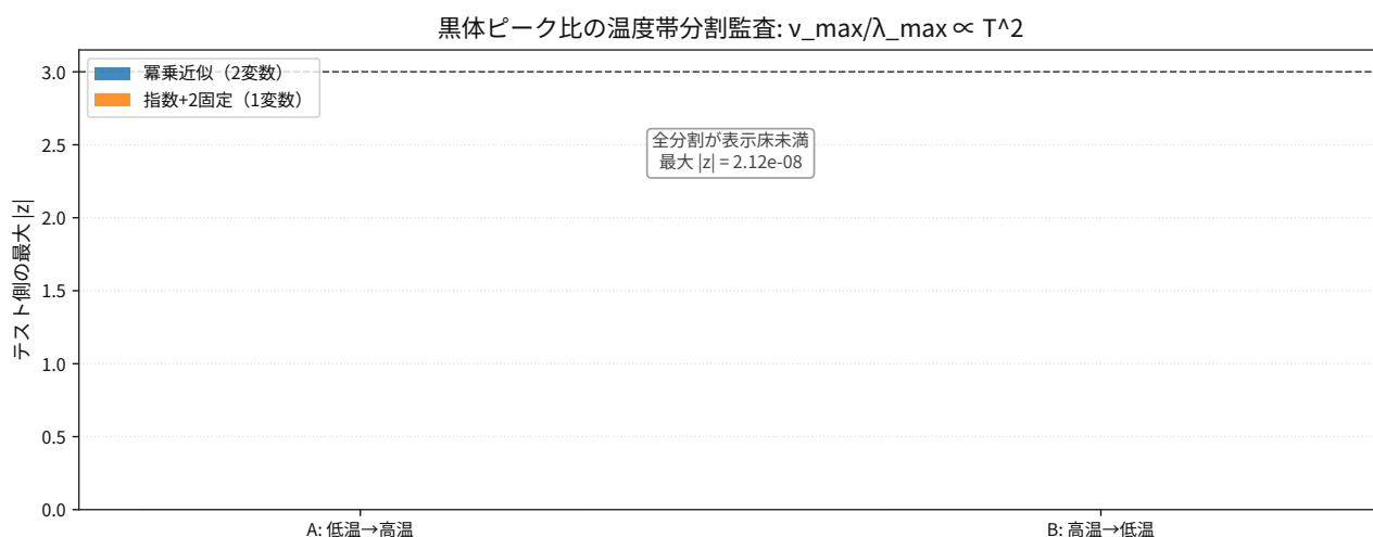
図 137: Comparison result for thermodynamics blackbody peak frequency per wavelength holdout splits.
