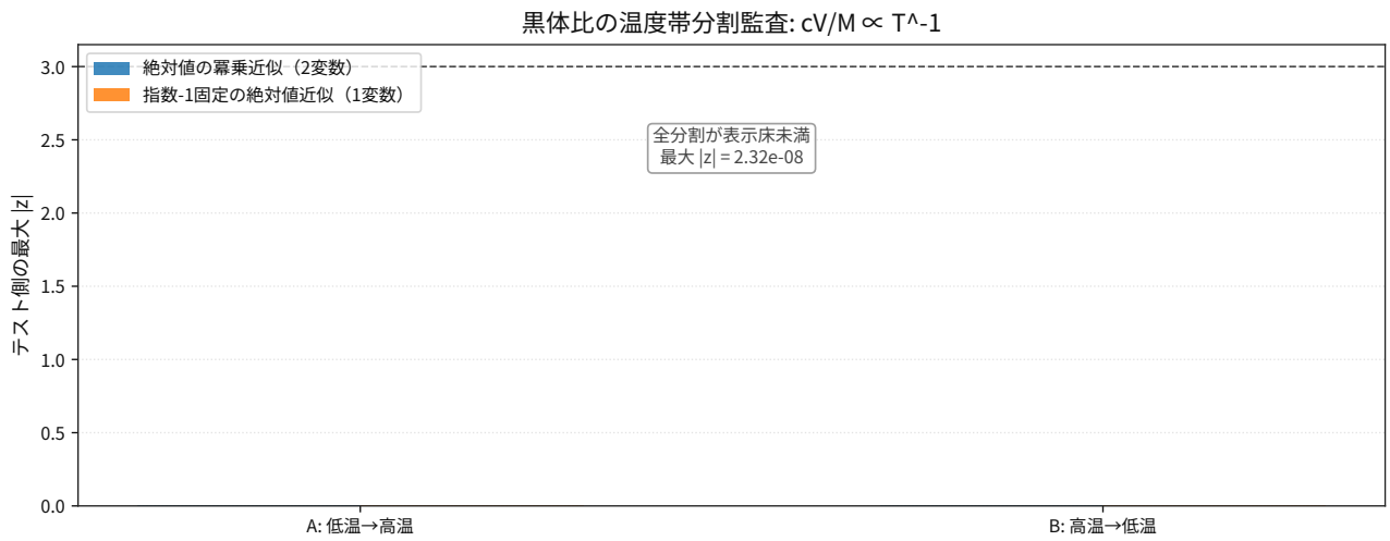
図 108: Comparison result for thermodynamics blackbody heat capacity flux ratio holdout splits.
