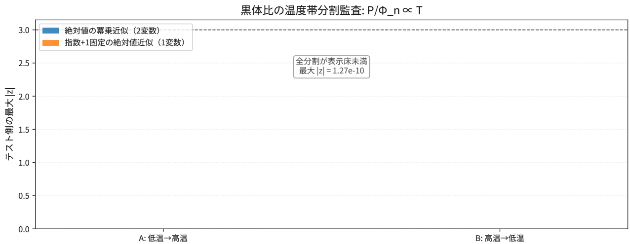
図 83: Comparison result for thermodynamics blackbody pressure per photon flux holdout splits.
