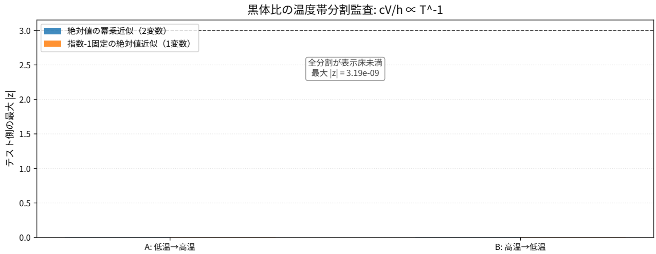
図 112: Comparison result for thermodynamics blackbody heat capacity enthalpy ratio holdout splits.
