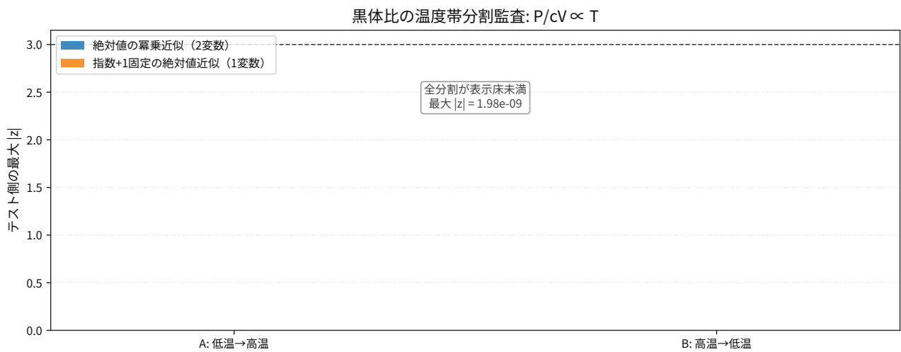
図 95: Comparison result for thermodynamics blackbody pressure per heat capacity density holdout splits.
