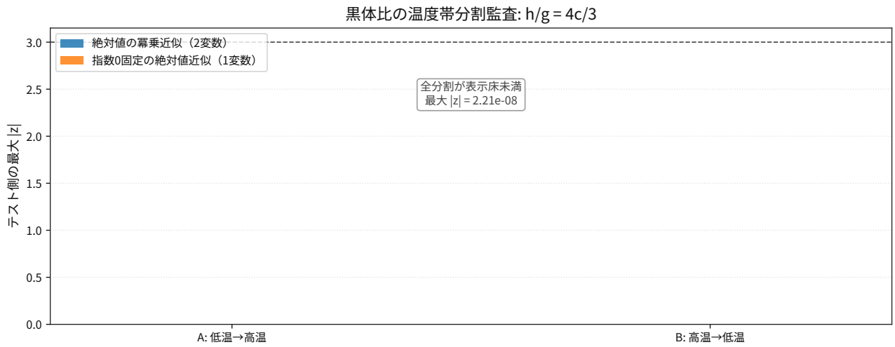
図 122: Comparison result for thermodynamics blackbody enthalpy momentum ratio holdout splits.
