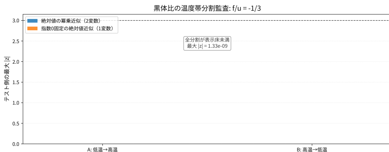
図 127: Comparison result for thermodynamics blackbody Helmholtz energy ratio holdout splits.
