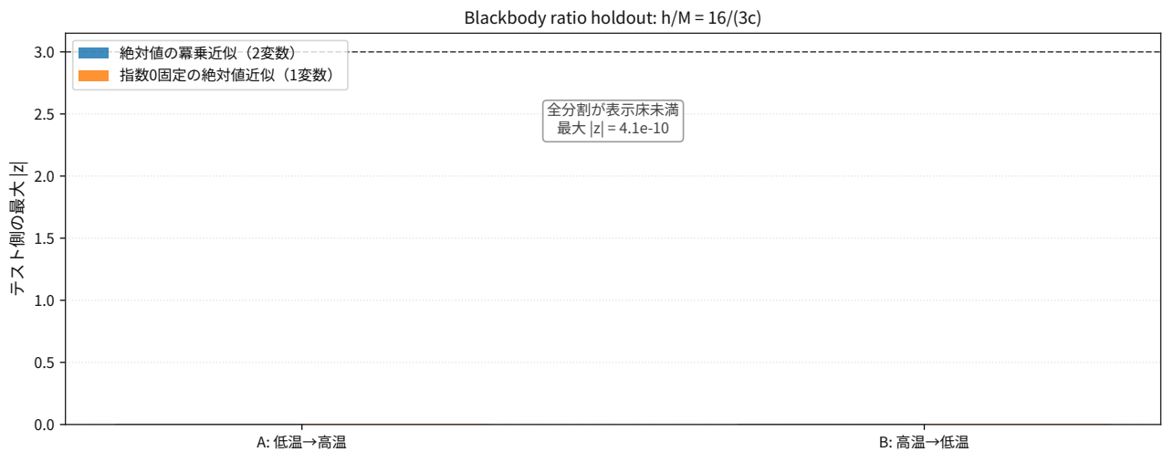
図 121: Comparison result for thermodynamics blackbody enthalpy flux ratio holdout splits.
