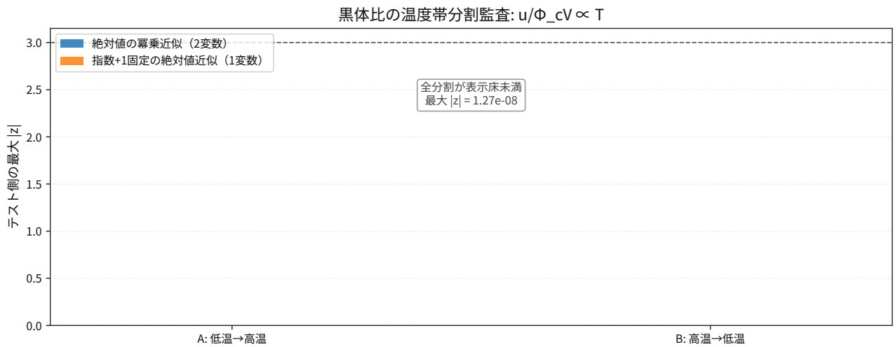
図 99: Comparison result for thermodynamics blackbody energy per heat capacity flux holdout splits.
