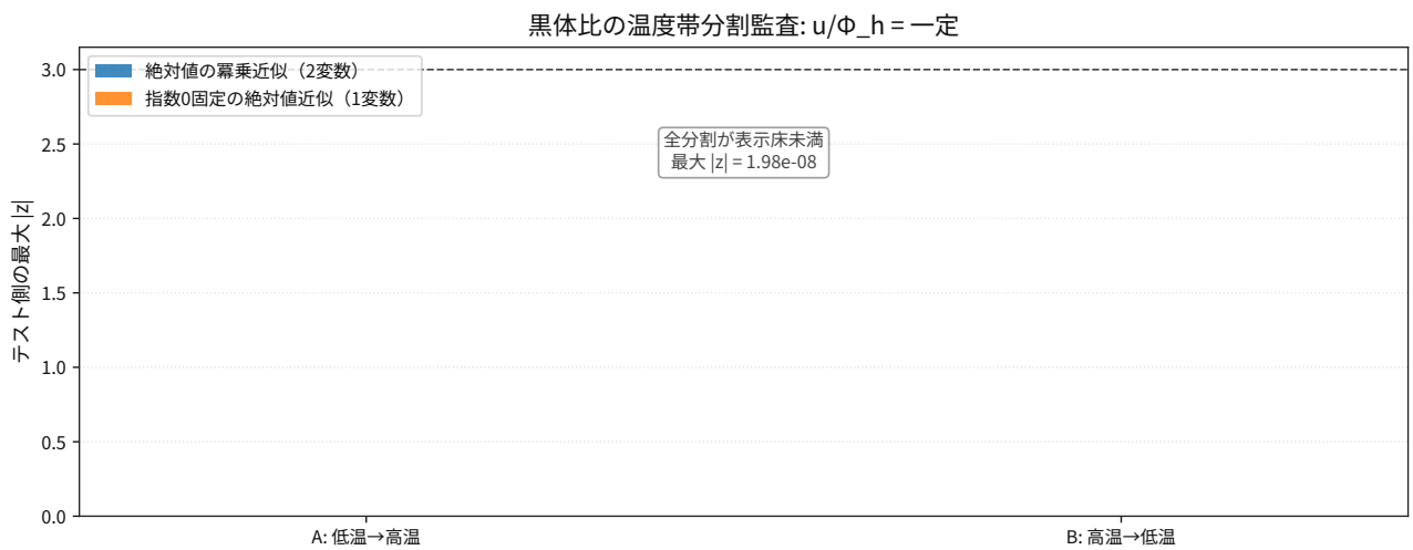
図 91: Comparison result for thermodynamics blackbody energy per enthalpy flux holdout splits.
