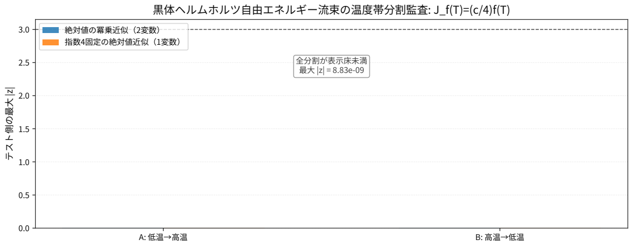
図 134: Comparison result for thermodynamics blackbody Helmholtz free energy flux holdout splits.
