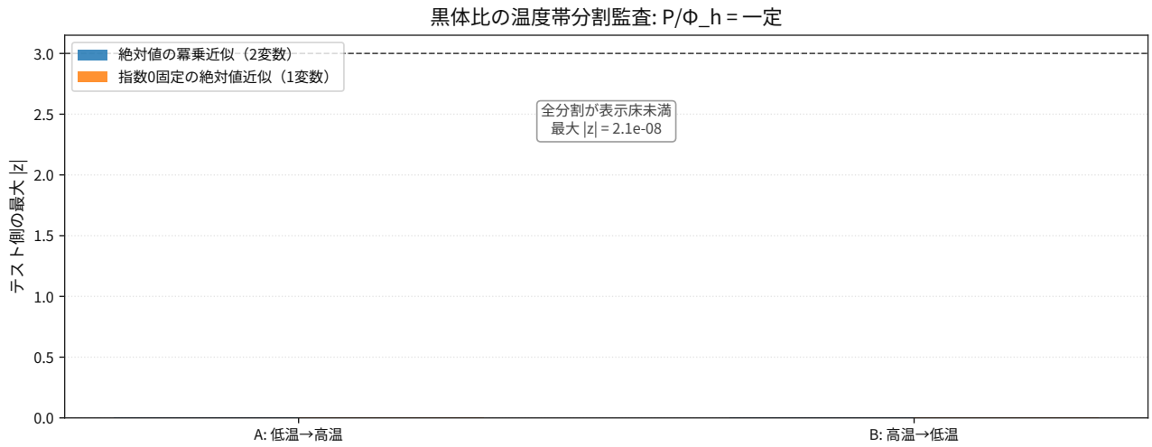
図 88: Comparison result for thermodynamics blackbody pressure per enthalpy flux holdout splits.
