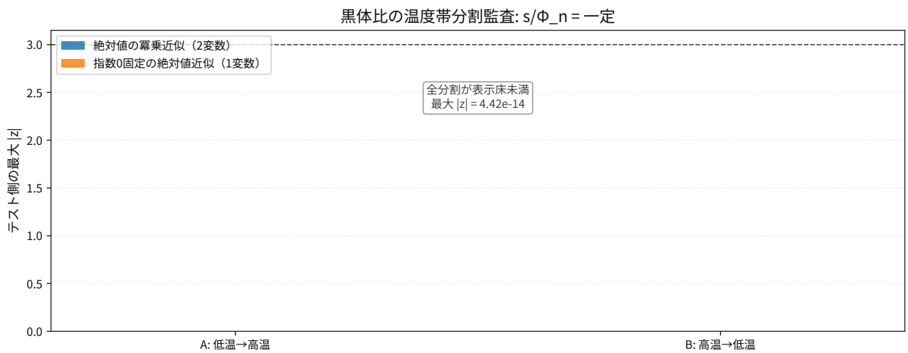
図 117: Comparison result for thermodynamics blackbody entropy per photon flux holdout splits.
