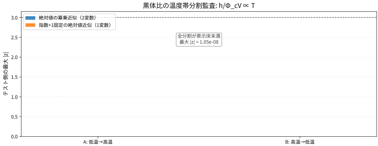
図 100: Comparison result for thermodynamics blackbody enthalpy per heat capacity flux holdout splits.
