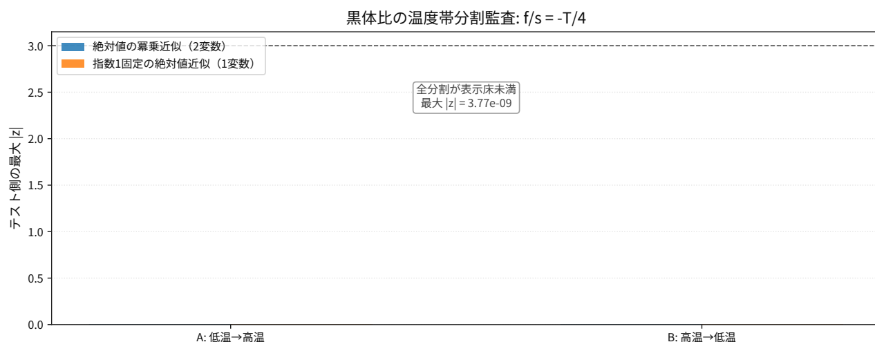
図 126: Comparison result for thermodynamics blackbody Helmholtz entropy ratio holdout splits.
