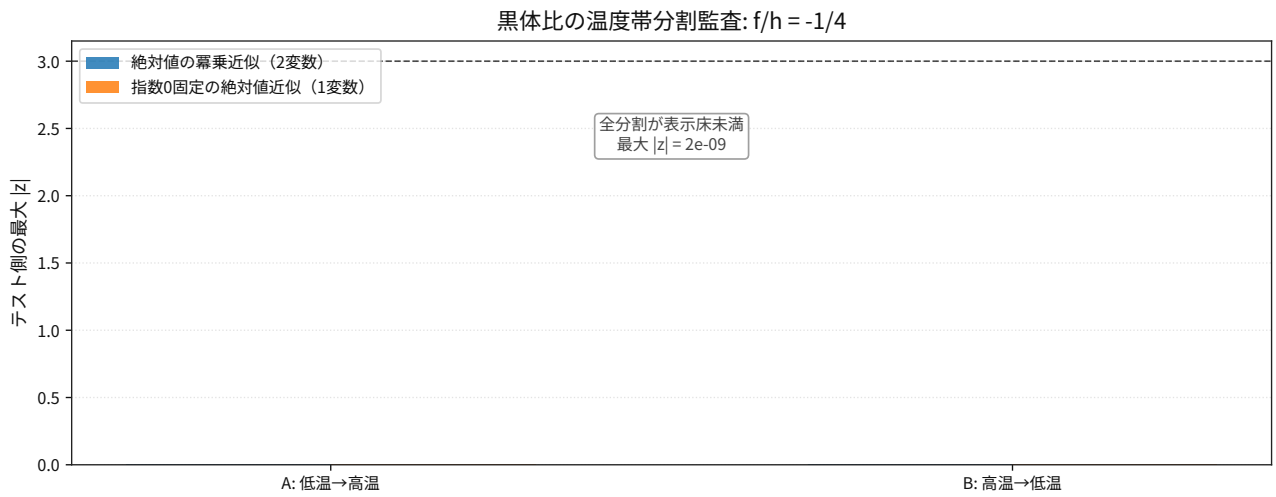
図 128: Comparison result for thermodynamics blackbody Helmholtz enthalpy ratio holdout splits.
