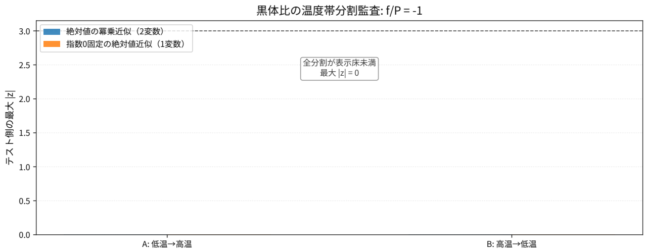
図 130: Comparison result for thermodynamics blackbody Helmholtz pressure ratio holdout splits.
