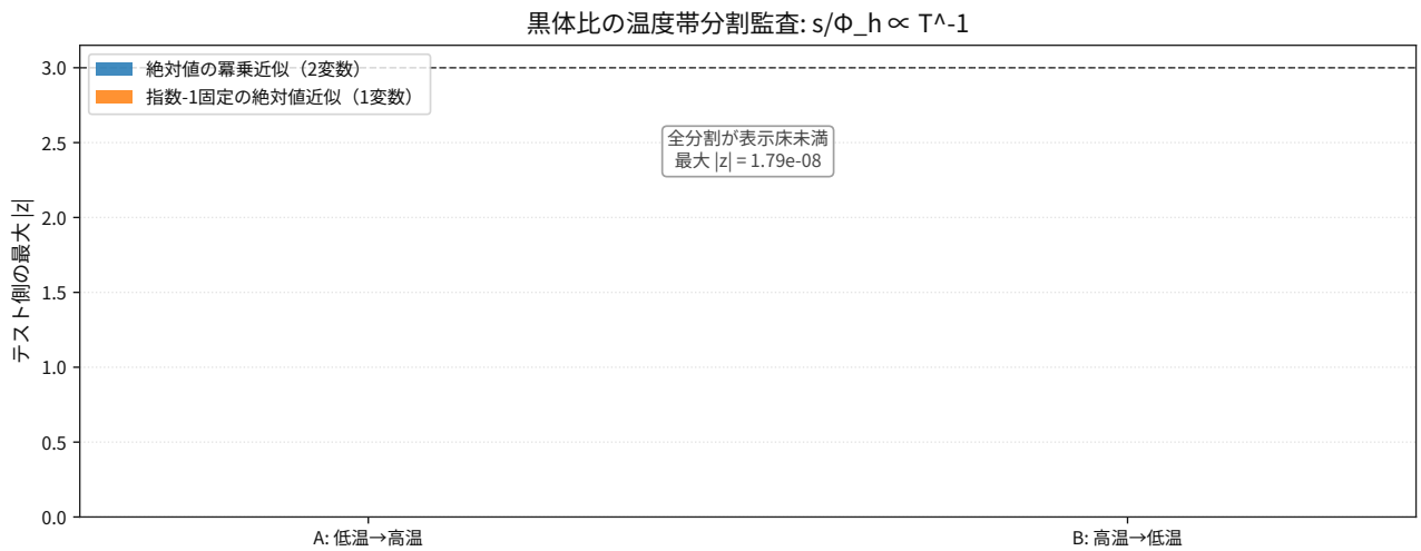
図 89: Comparison result for thermodynamics blackbody entropy per enthalpy flux holdout splits.
