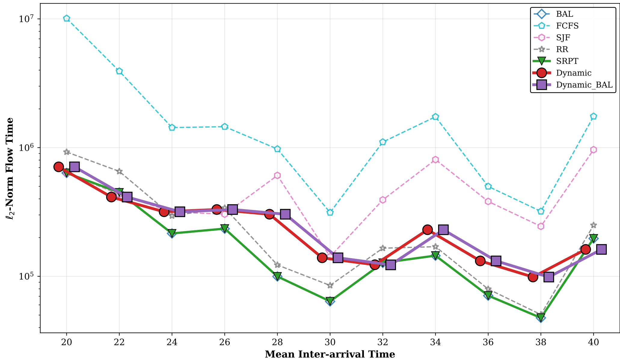
Clairvoyant \ell_2 -Norm Comparison Bounded Pareto ( H = 2^{18} , H/L \approx 64359 )
