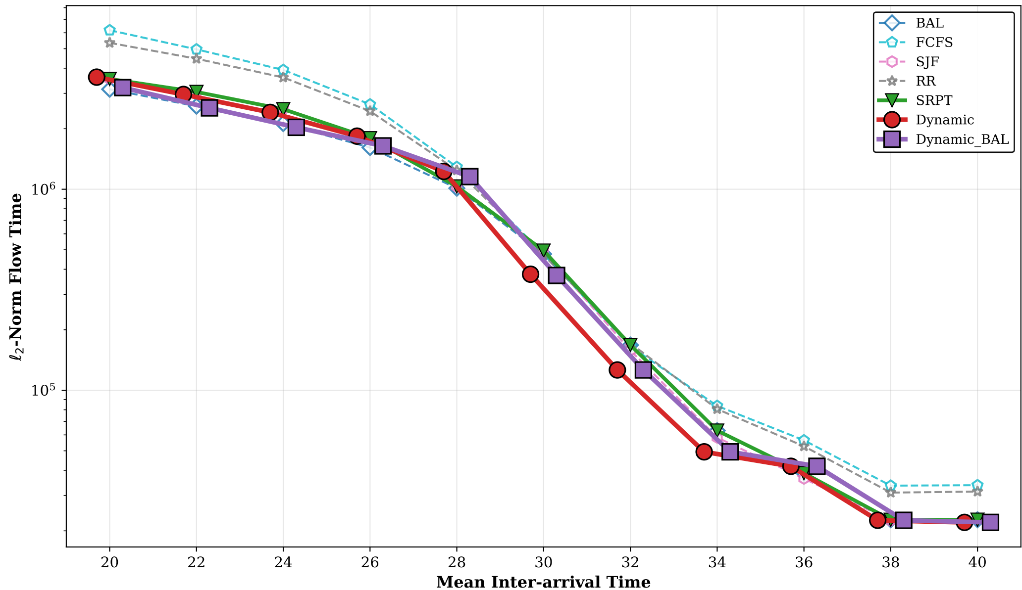
Clairvoyant \ell_2 -Norm Comparison Bounded Pareto ( H = 2^9 , H/L \approx 65 )
