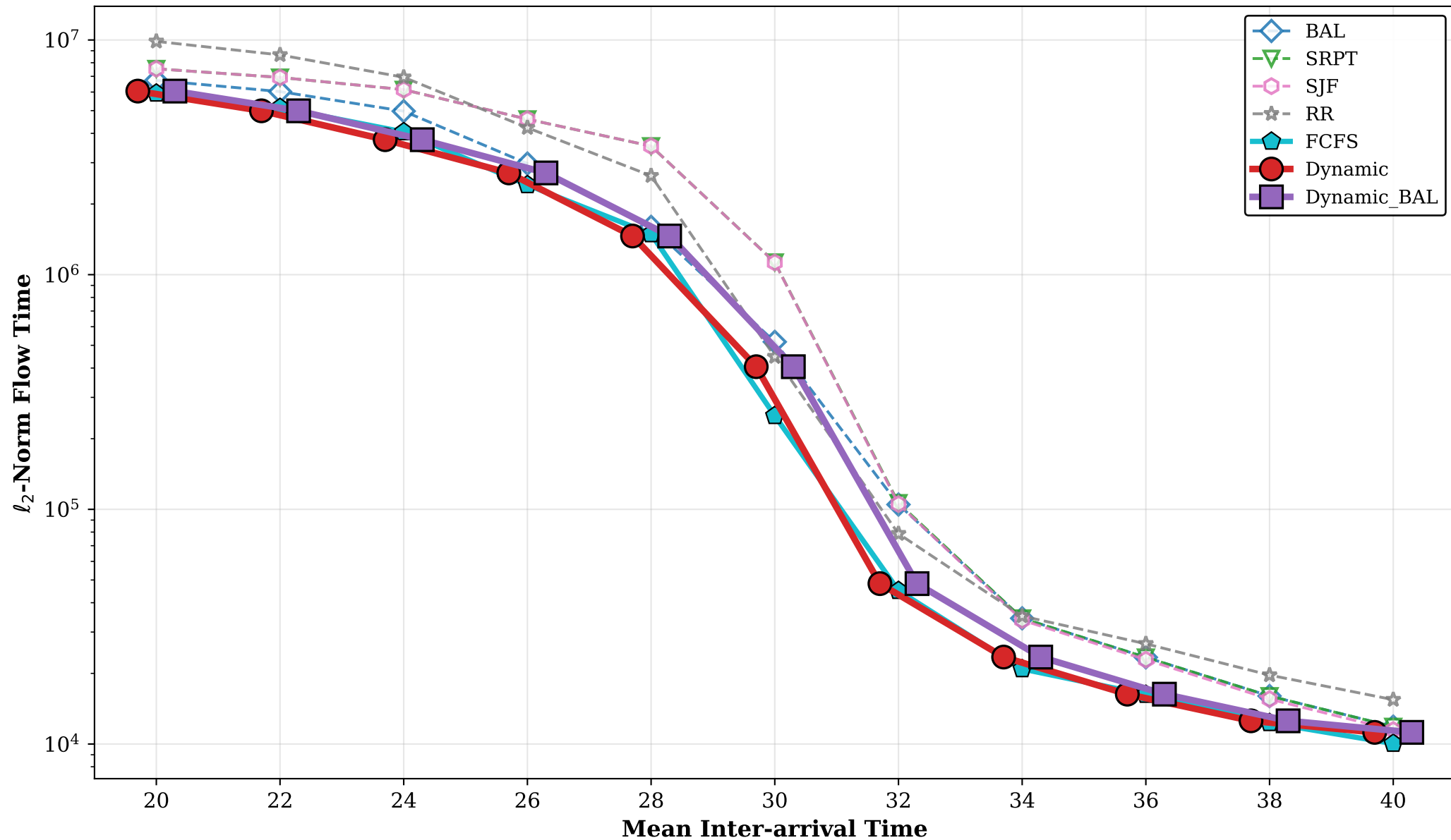
Clairvoyant \ell_2 -Norm Comparison Normal ( \mu = 30, \sigma = 12, CV=0.40 )
