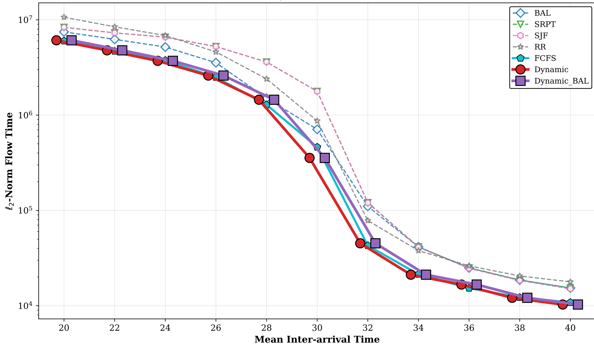
Clairvoyant \ell_2 -Norm Comparison Normal ( \mu = 30, \sigma = 6, CV=0.20 )
