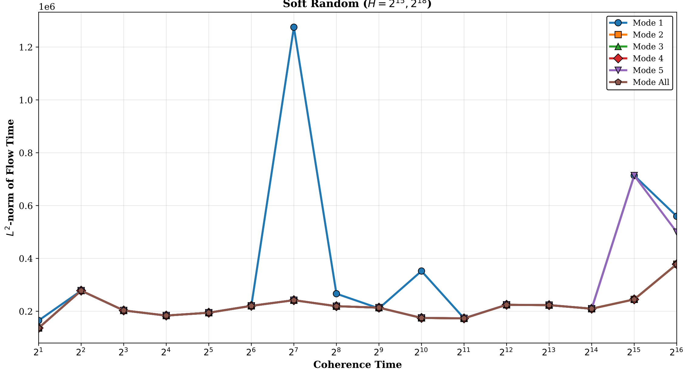
Dynamic_BAL Mode Comparison Soft Random ( H = 2^{15}, 2^{18} )
