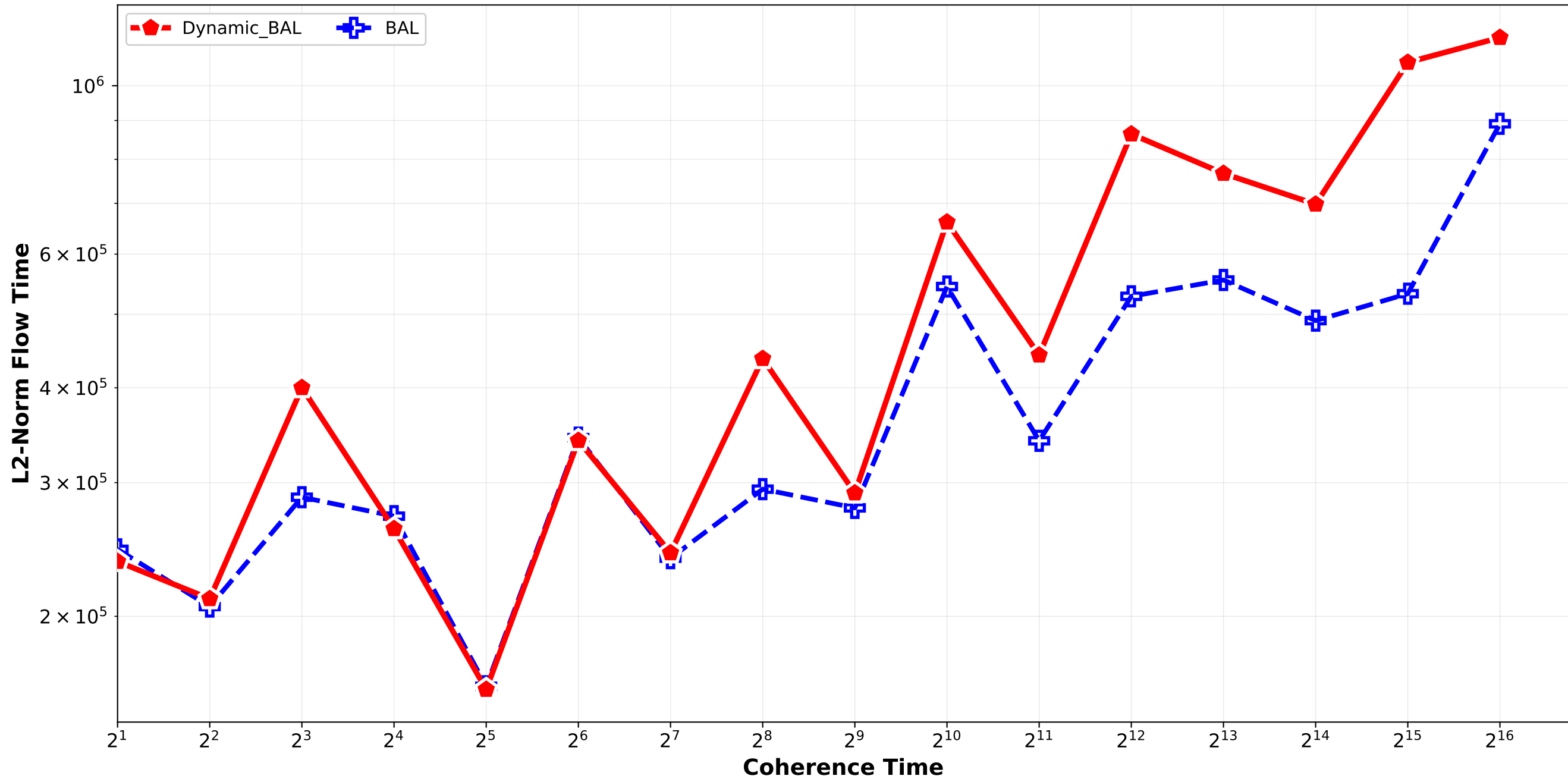
Dynamic_BAL vs BAL - L2 Norm Flow Time Bounded_Pareto_combination_random H64_H512_H4096_H32768 / quadruplet_1
