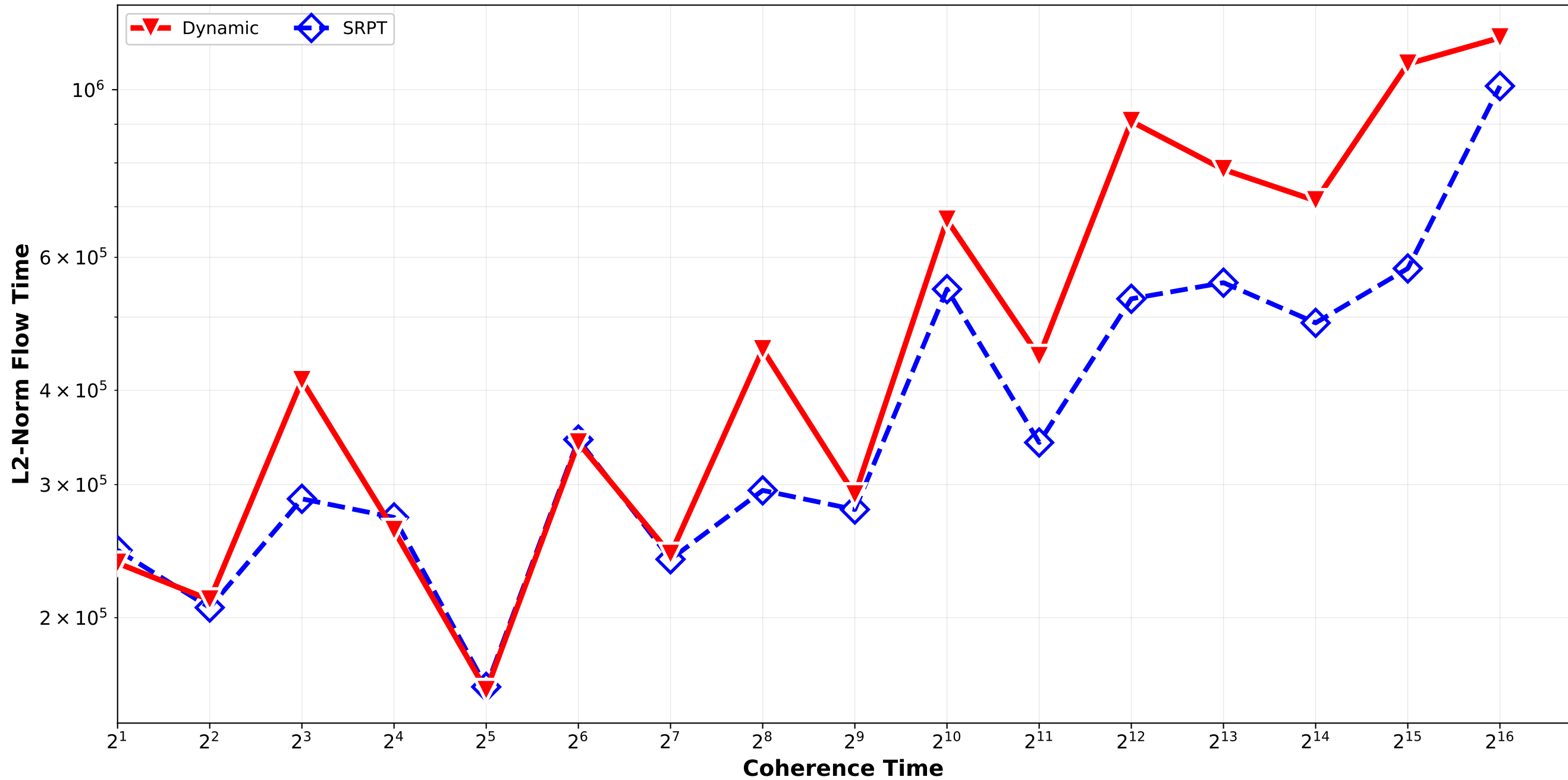
Dynamic vs SRPT - L2 Norm Flow Time Bounded_Pareto_combination_random H64_H512_H4096_H32768 / quadruplet_1
