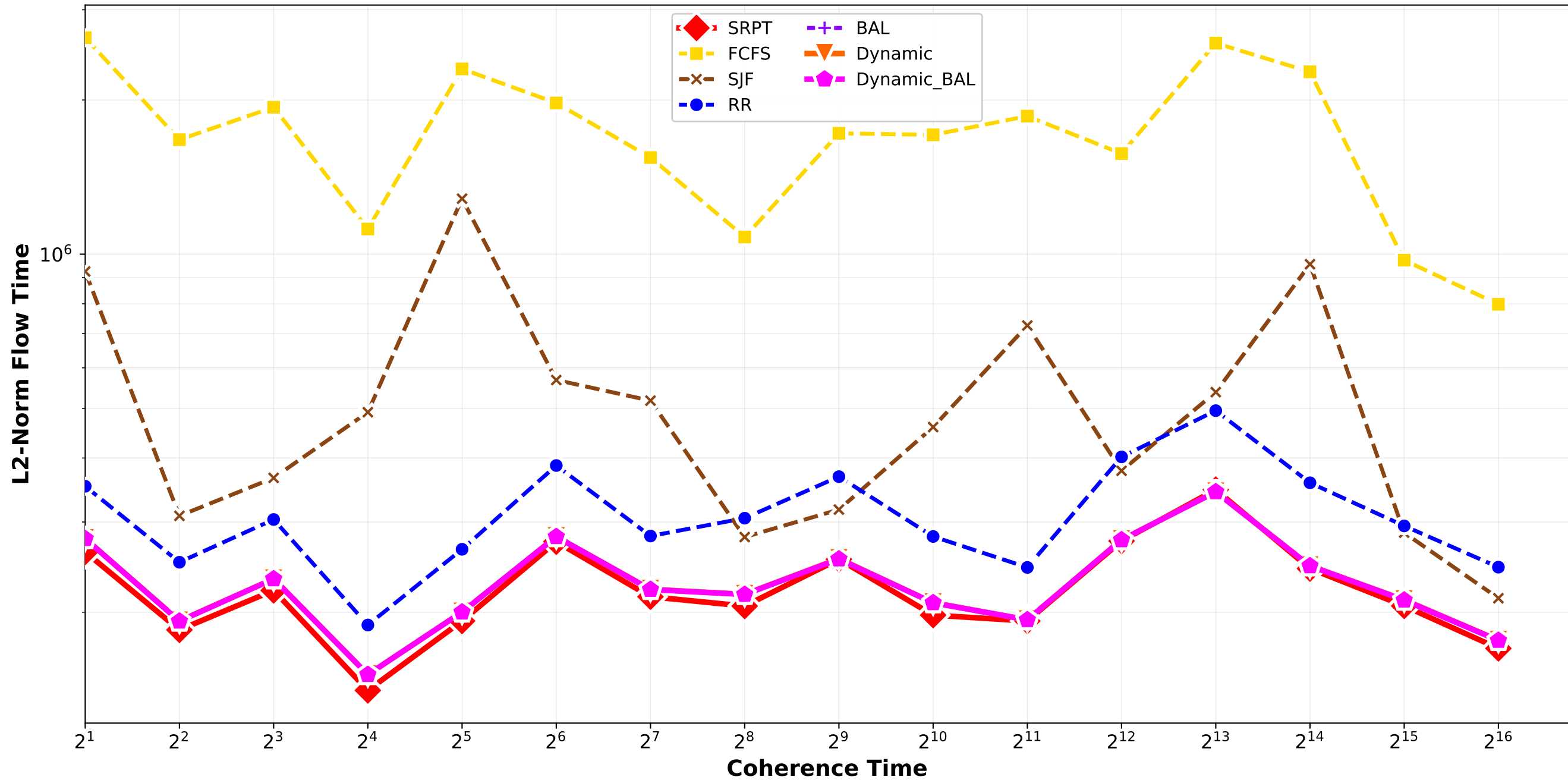
Clairvoyant Algorithms - L2 Norm Flow Time Bounded_Pareto_combination_random H4096_H32768_H262144 / triplet_3
